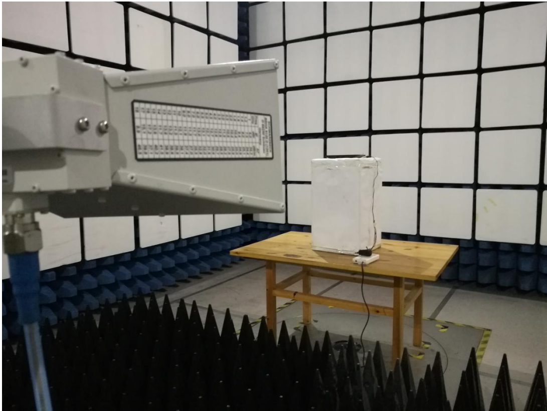
Above 1GHz
