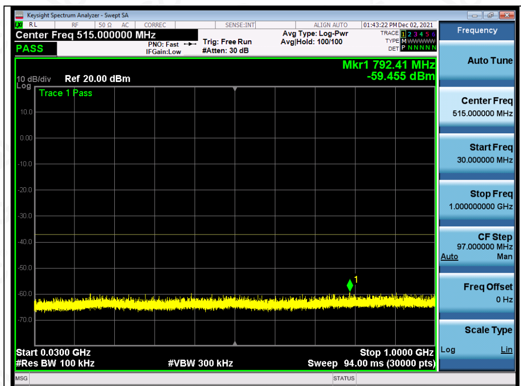
Test_Graph_802.11n40_ANT1_5190_MCS0_Frequency Band 1
