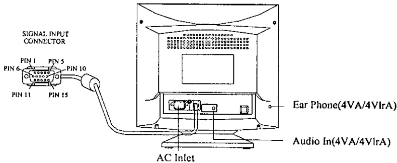
Figure 2 Connecting Cables
