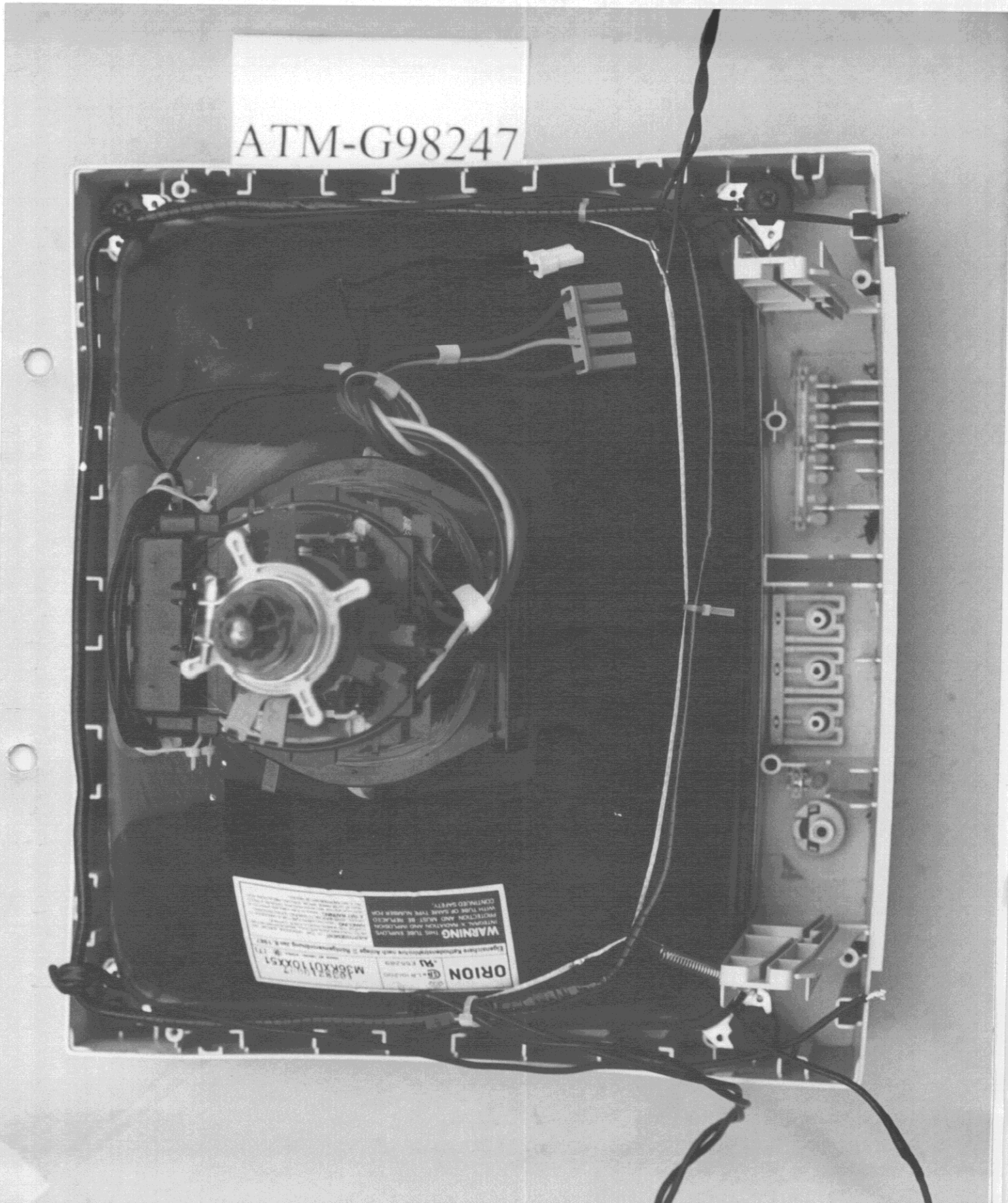
Figure 4 Frame of CRT (internal View)
