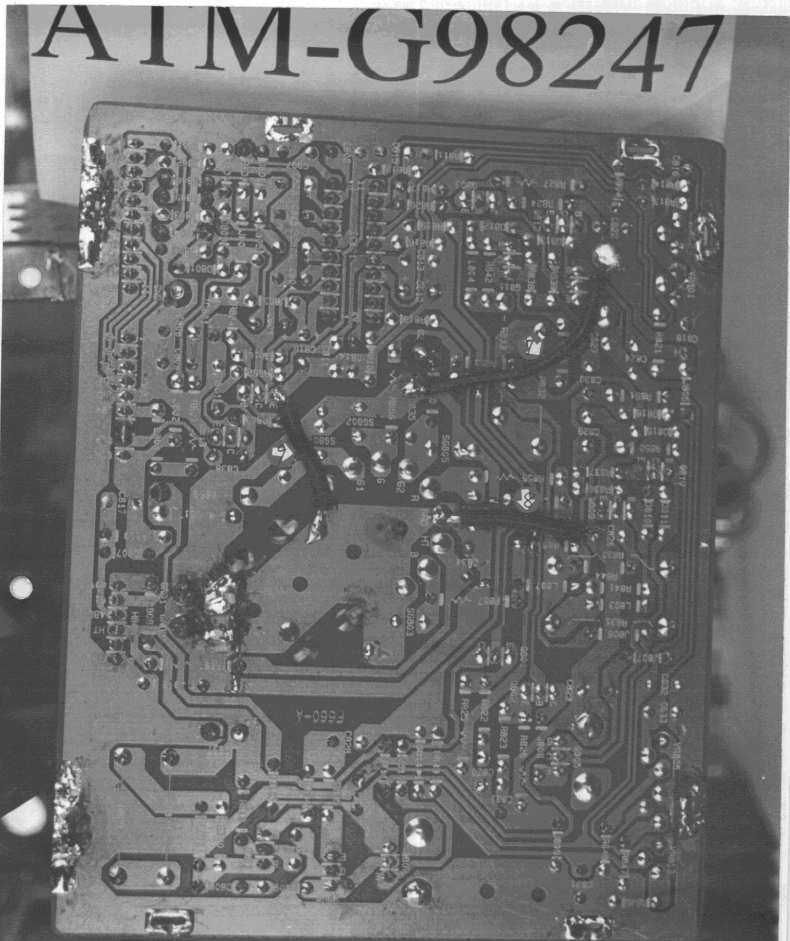
Figure 8 Video Board (Solder Side)
