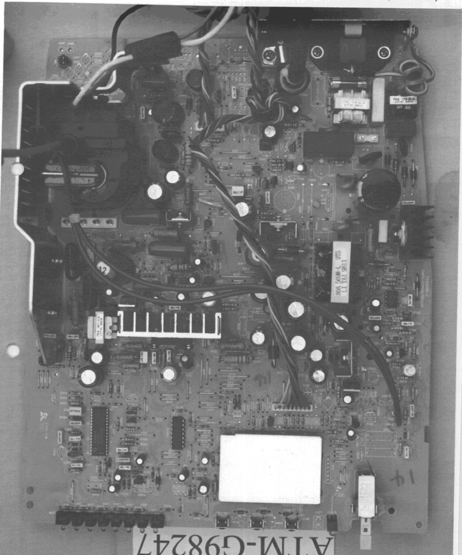
Figure 5 Main Board (Component Side)
