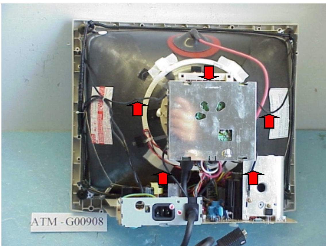
Figure 6 Frame of CRT (Internal View)
