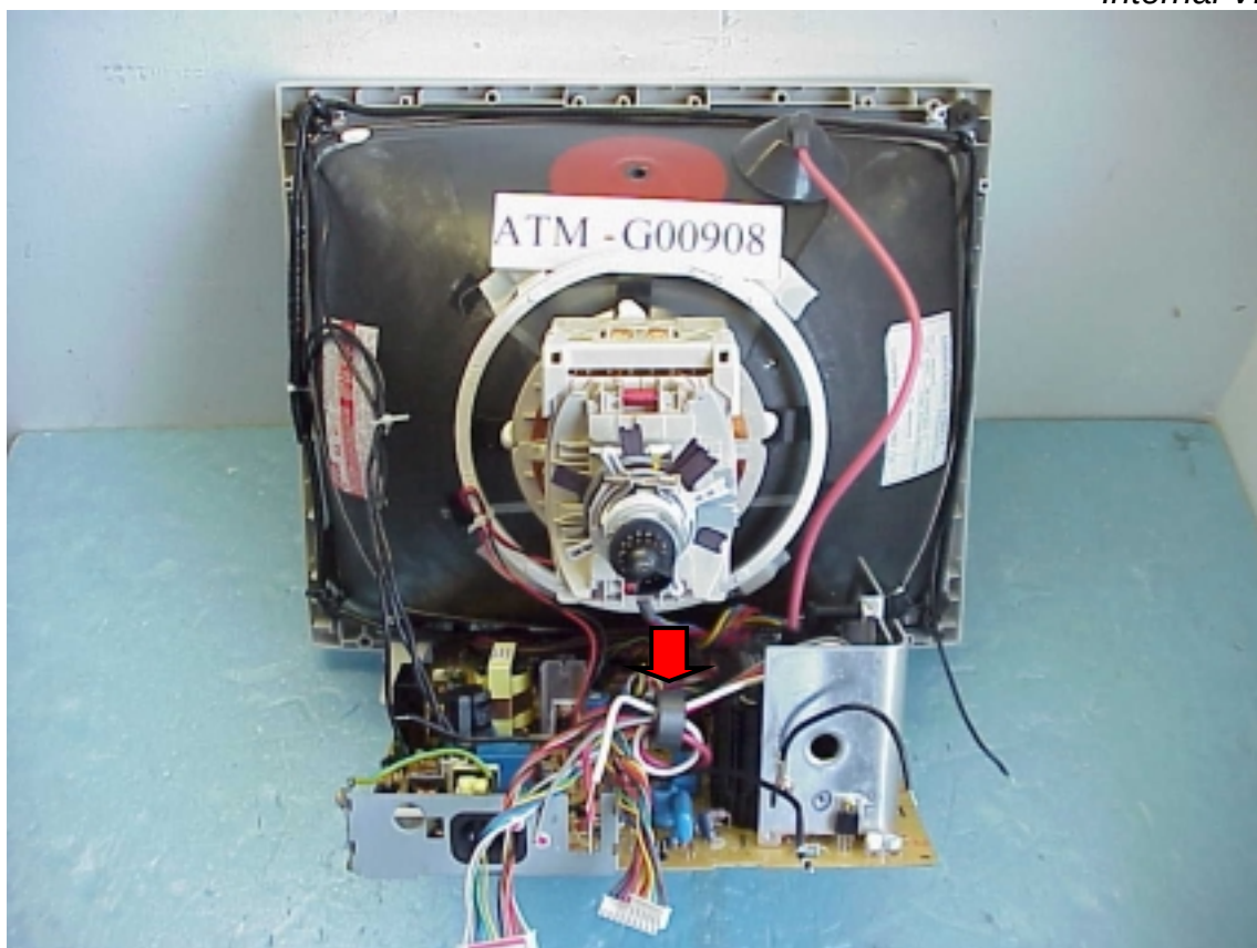
Figure 5 Internal View
