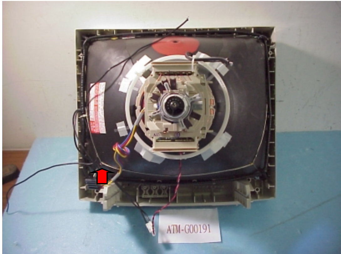
Figure 4. Frame of CRT (Internal View)
