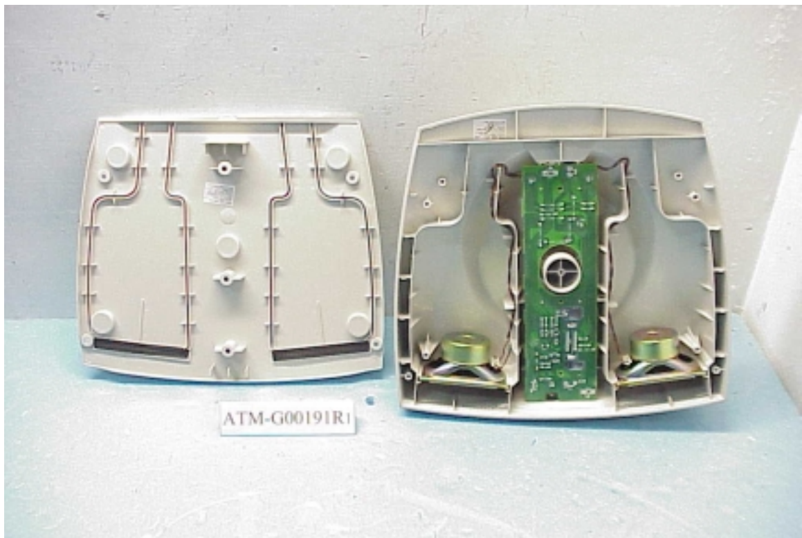
Figure 11 Internal View of Audio Base
