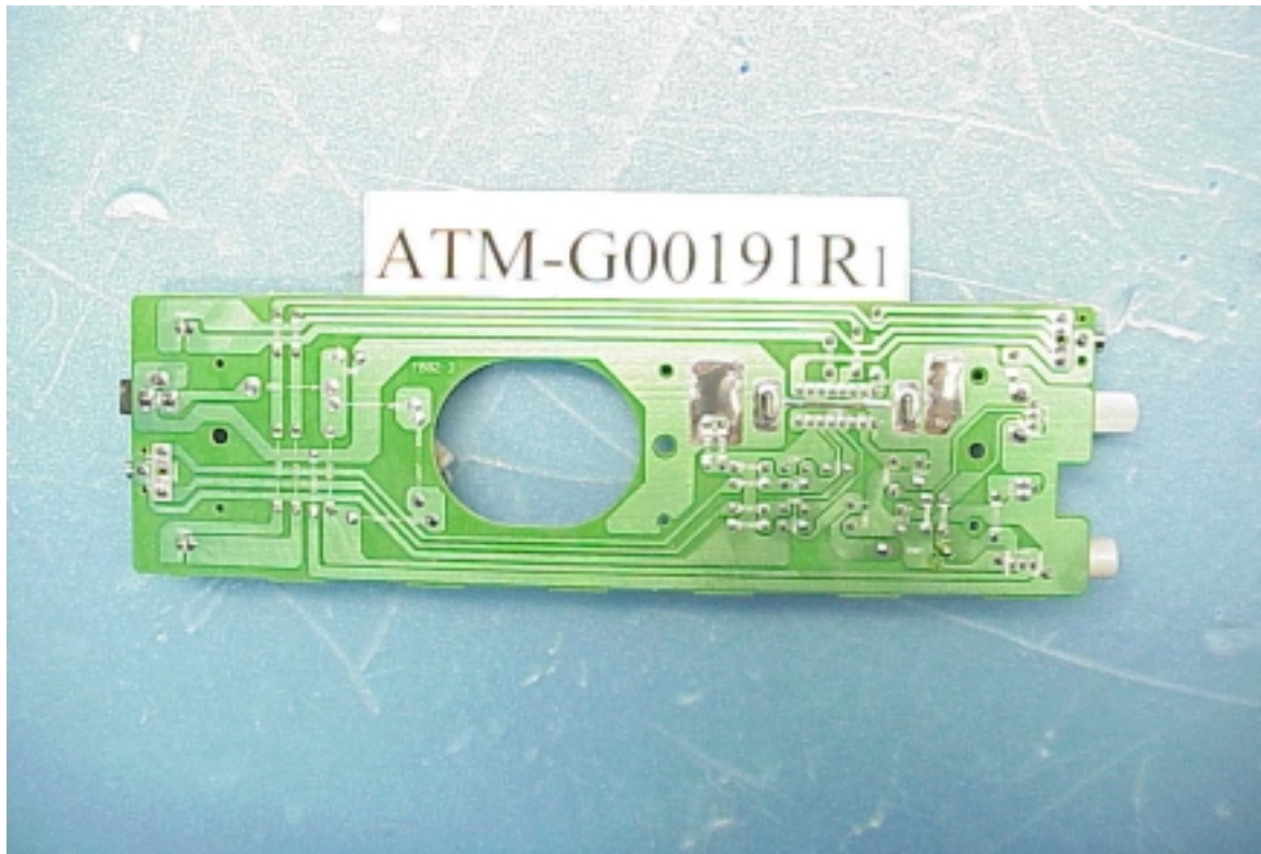
Figure 13 Control Board of Audio Base
