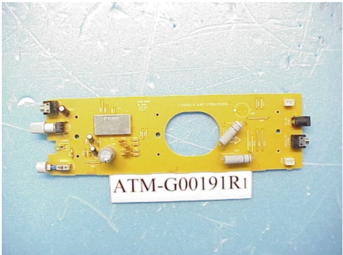
Figure 12 Control Board of Audio Base
