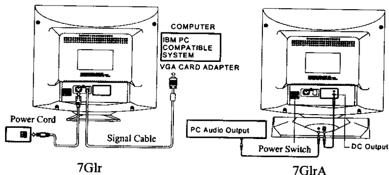
Figure 2 Connecting Cables
