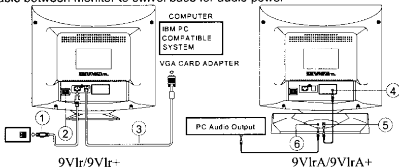
Figure 2 Connecting Cables
