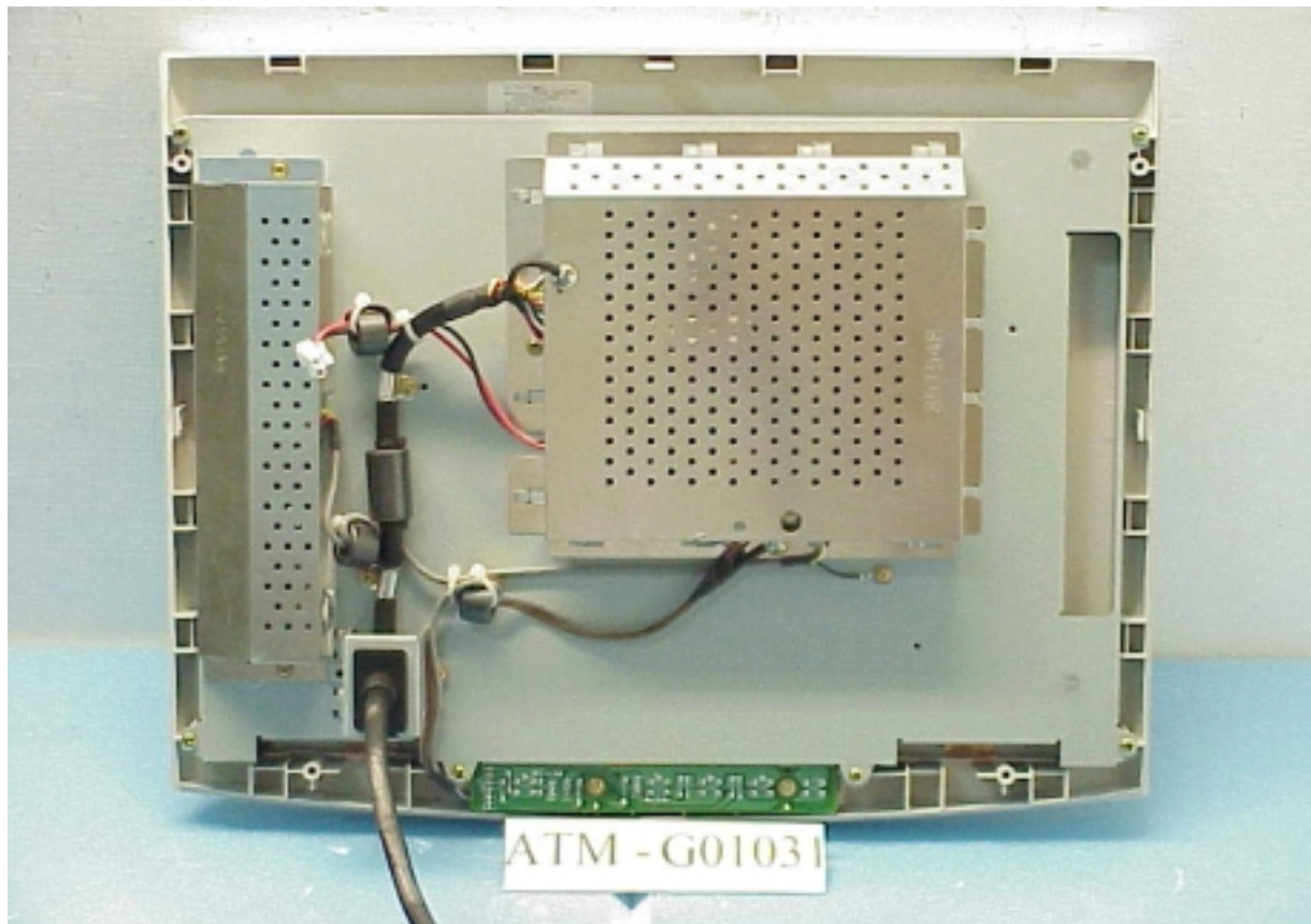
Figure 3 Internal View (Removed Back Cover)
