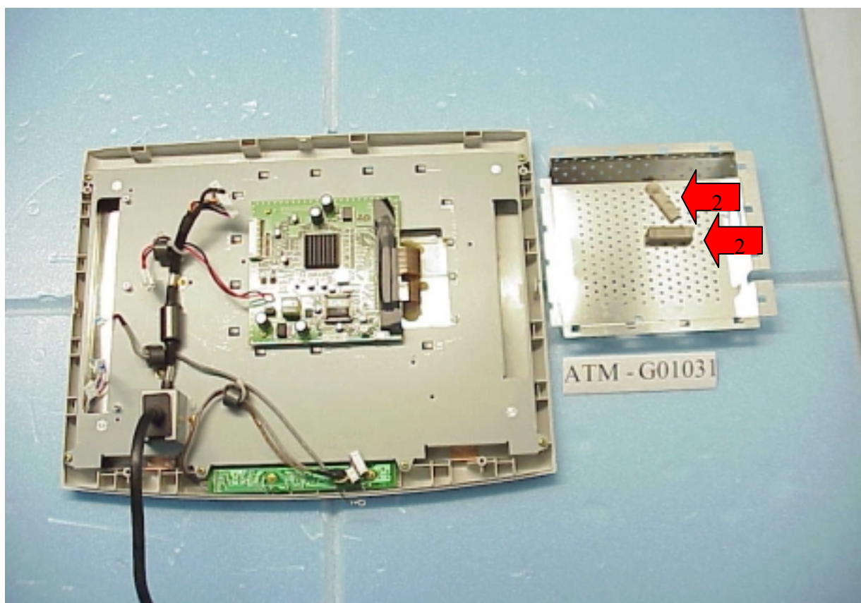
Figure 4 Internal View
