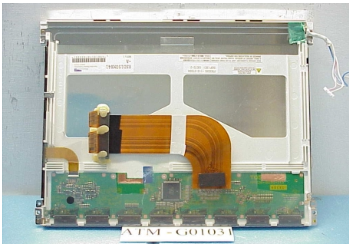
Figure 6 Toshiba LCD Panel (Rear View)
