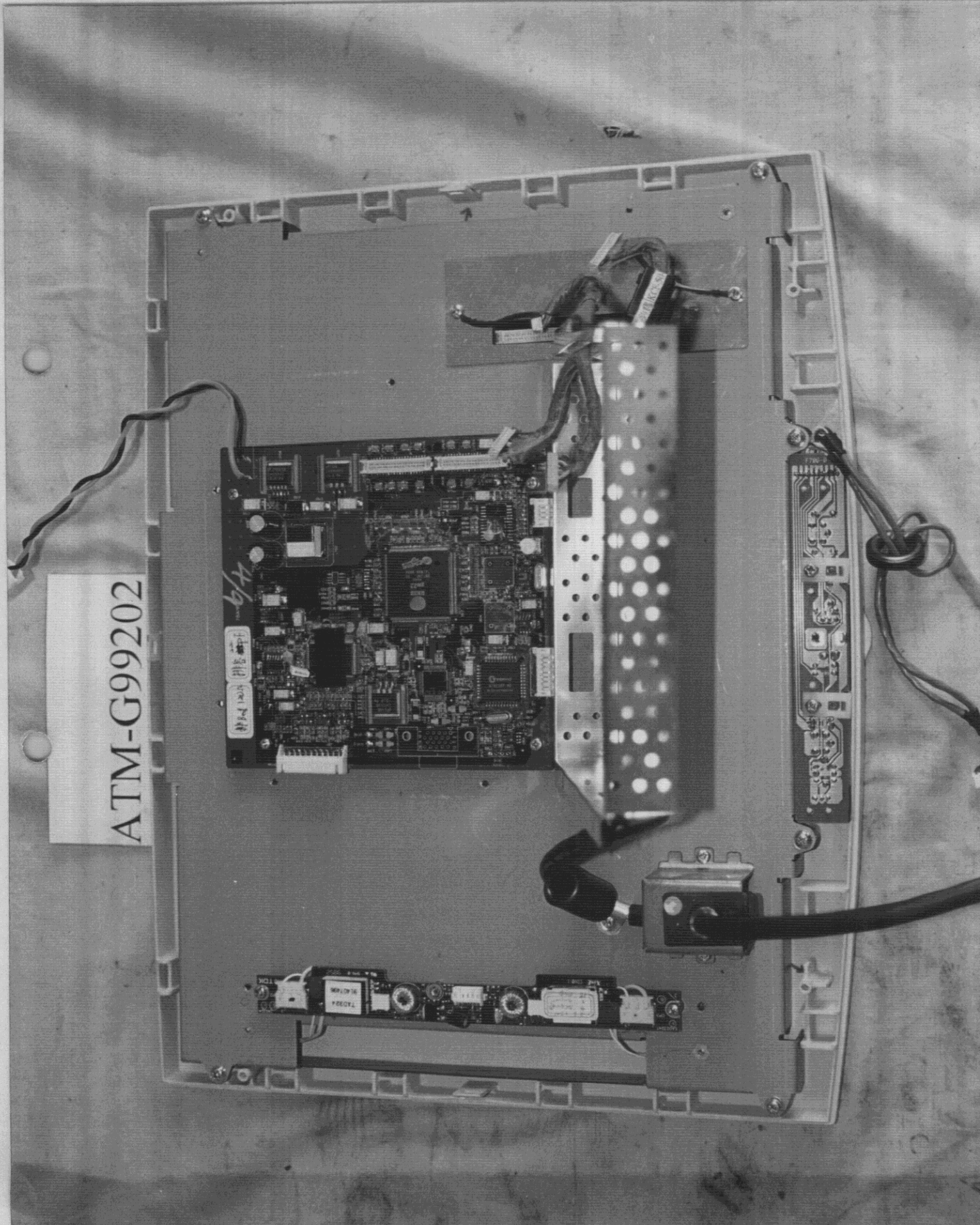
Figure 6 Internal View of EUT w/ LG LCD Panel
