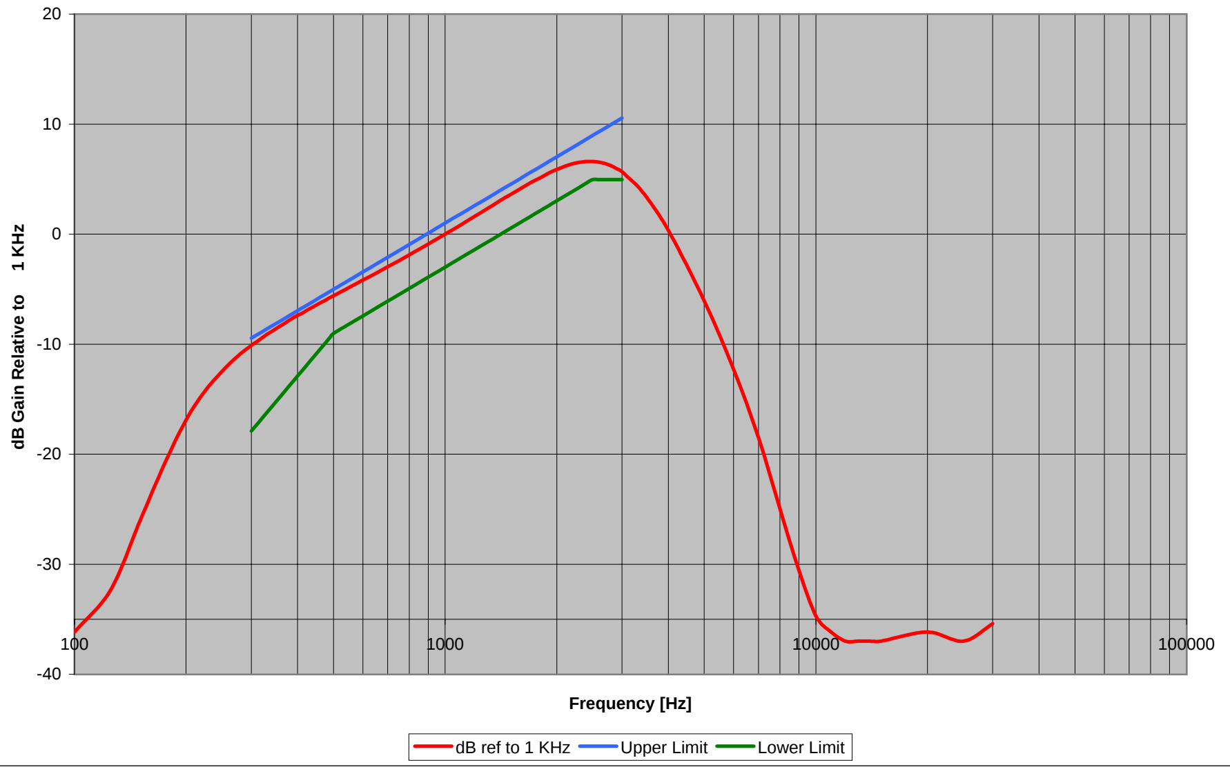
RPU 416TX Audio Response Wide Band
