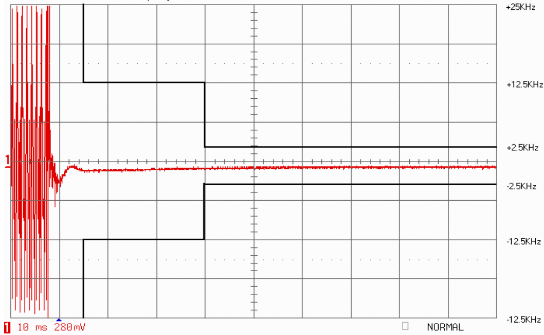
RPU 416 Transient Frequency Behavior Narrow Band Switch On Condition
