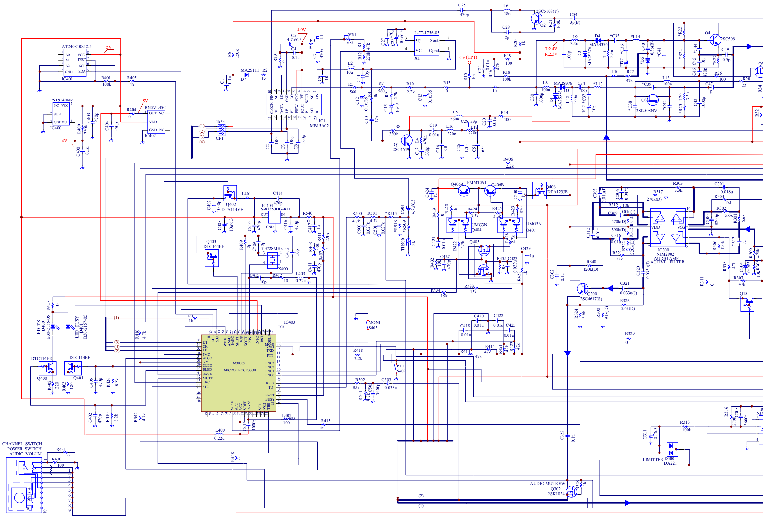
RPU416B Schematic Diagram
