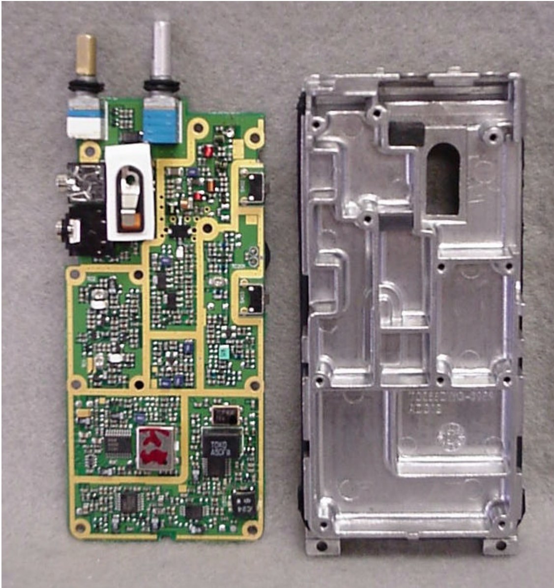
Photo 8. EUT, Top Side, Showing Shield Removed
