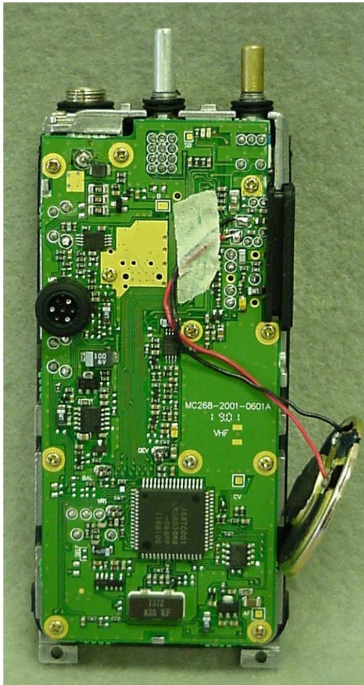
Photo 7. EUT, Bottom Side of Main Board
