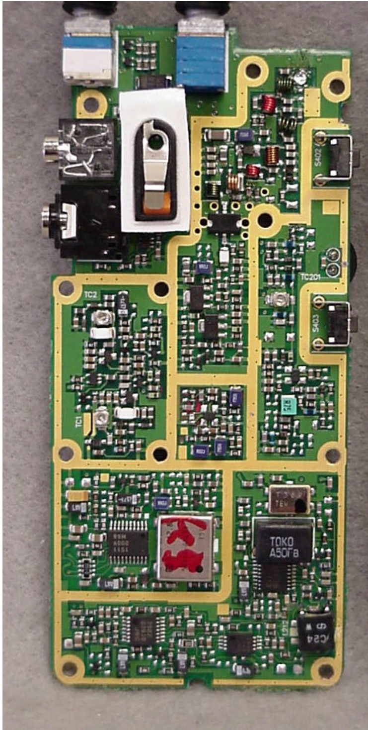
Photo 9. EUT, Top Side of Main Board
