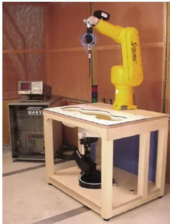
DASY3 SAR Measurement System with SAM phantom
