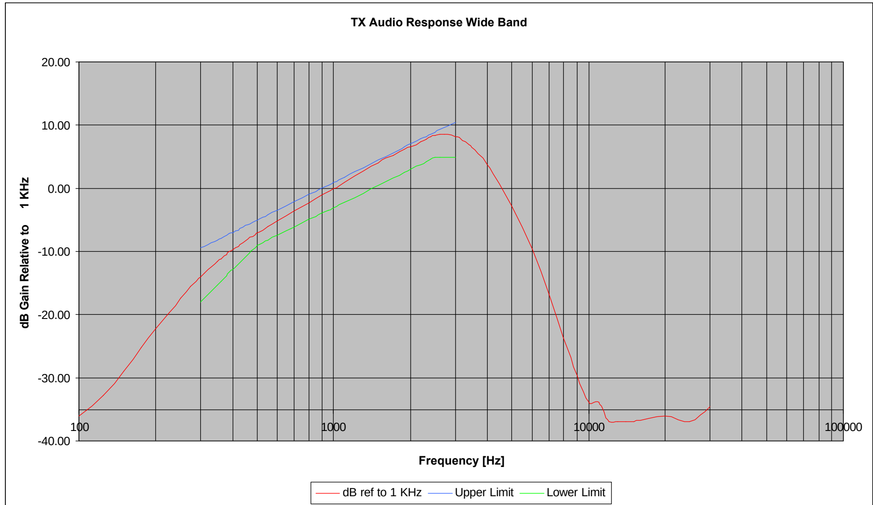
Figure 4d. Modulation Characteristics
