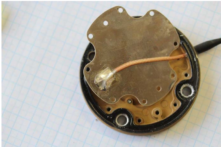
AT2400-2W-TNCM-008-00-05-L inside (rear) - feedline
