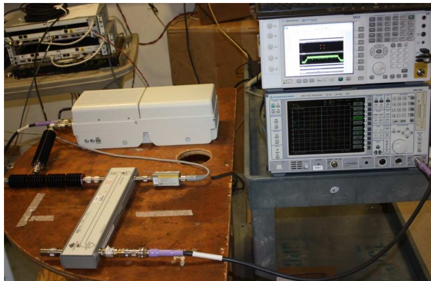
Figure 10.2 Setup Photo of Conducted Emissions Test at Antenna Ports.
