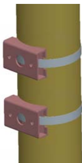
Figure 3-2 Pole-mount bracket attachment to a large pole
