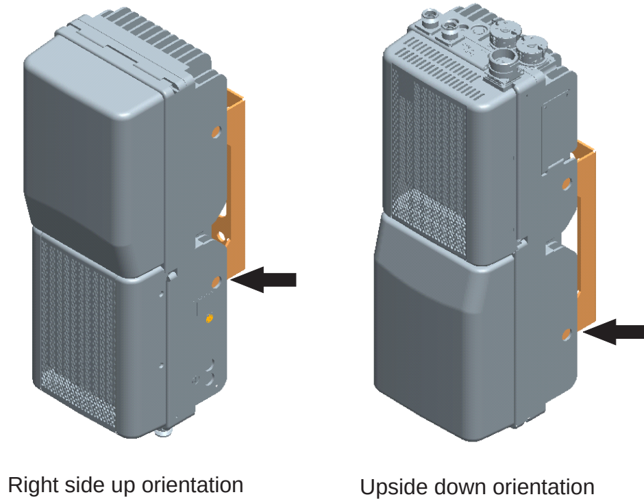
Figure 3-9 Lower screws for attachment to wall-mount bracket
