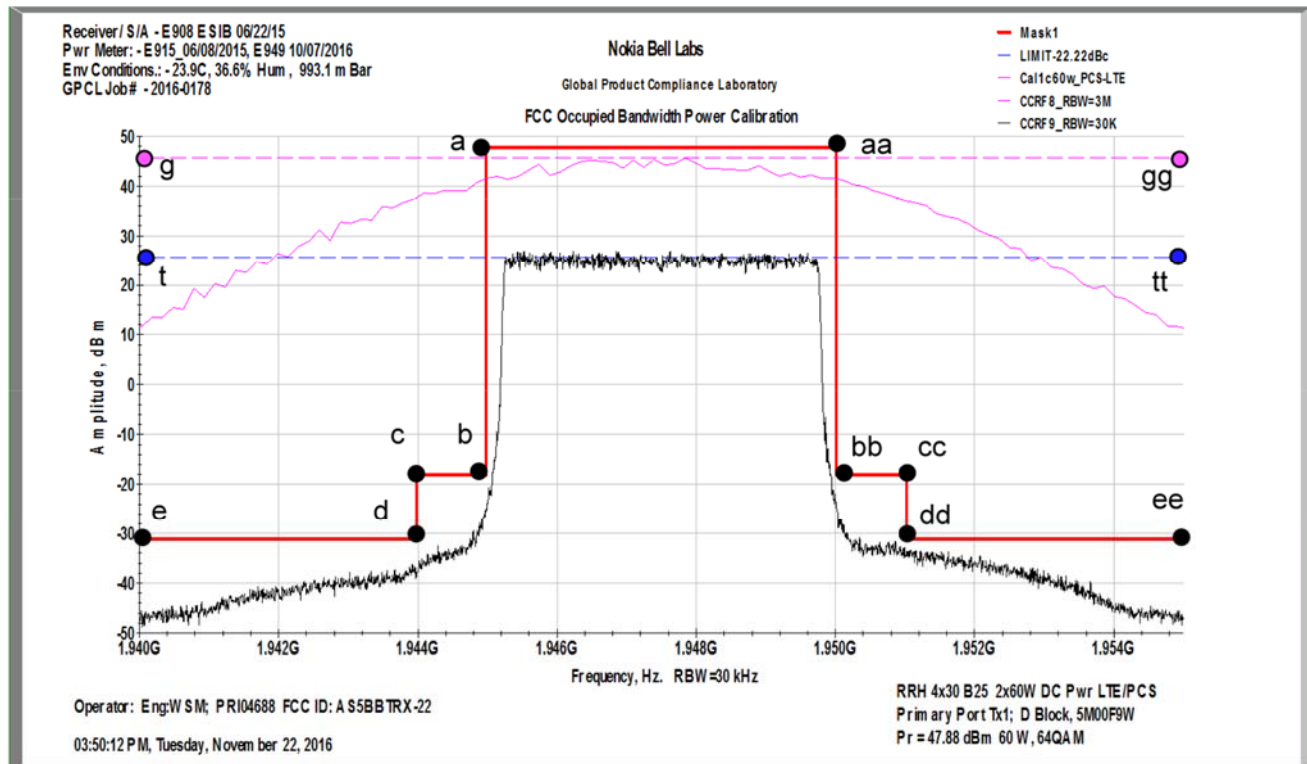
Figure 4.3.2.3 Mask Parameters
