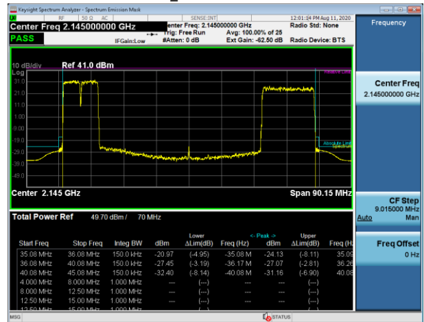
OOBE_TM3_1_3C_5+5+15MBW_2112_2117_2172_TX1 90W_LTE+LTE+5G-NR
