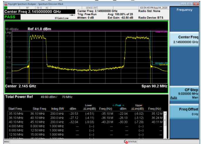
OOBE_TM3_2_2C_10+15MBW_2115_2172_TX1 90W LTE+5G-NR
