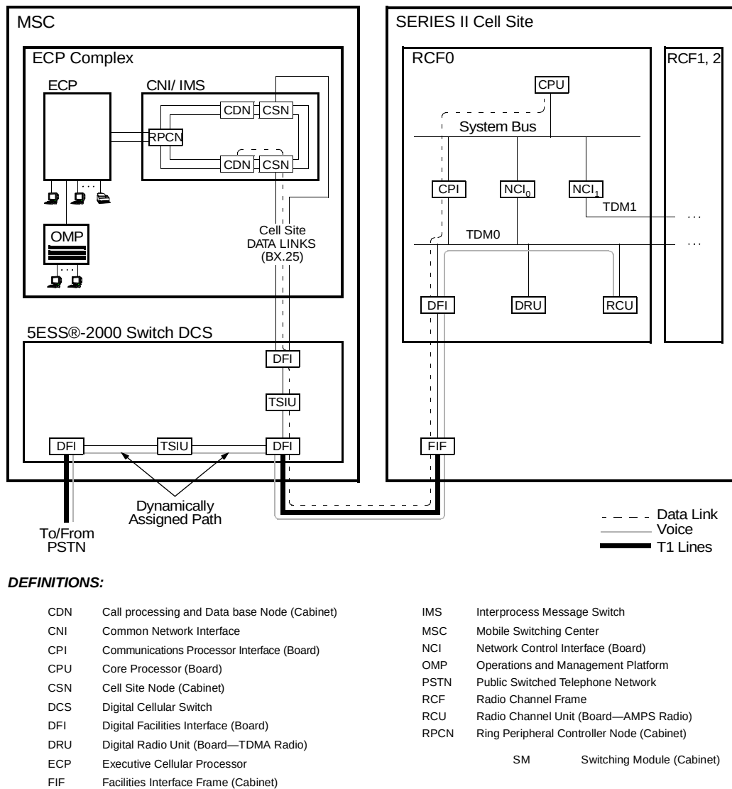
Figure 11-6. Data Link and Voice Paths—Example
