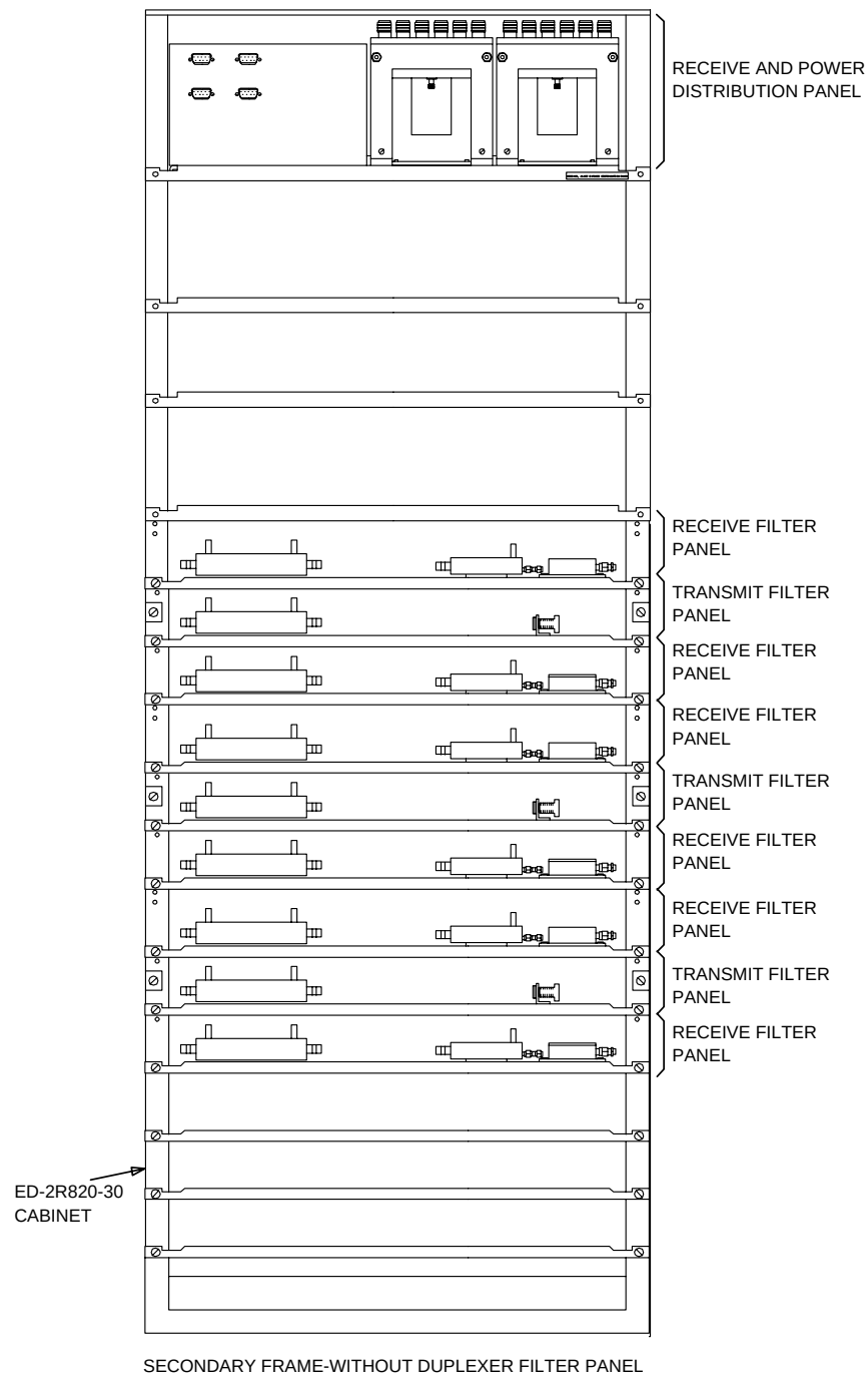
Figure 8-34. Growth Antenna Interface Frame J41660F-2
