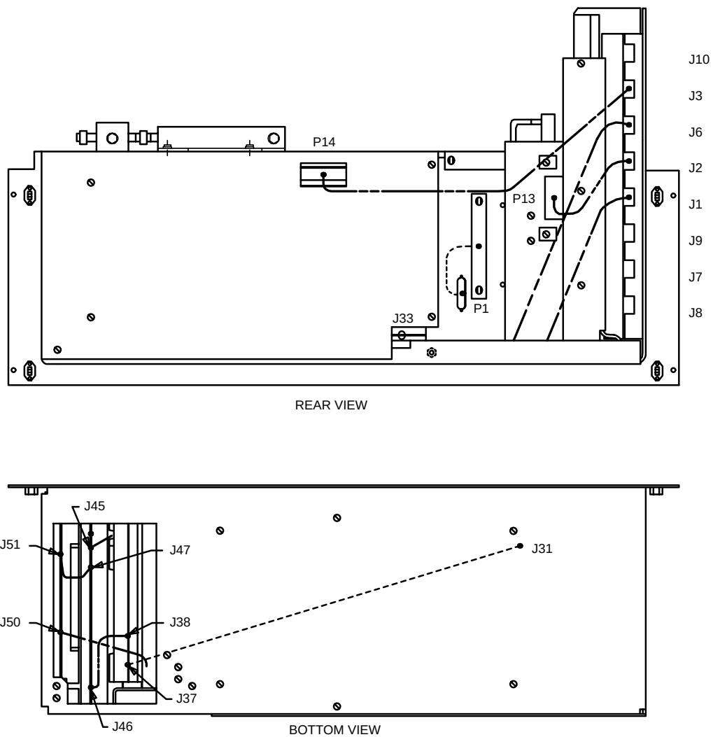
Figure 8-22. Linearizer Unit ED-2R841-30
