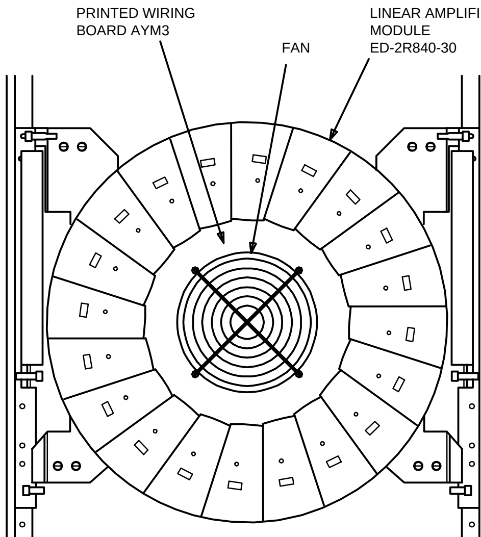
FRONT VIEW
