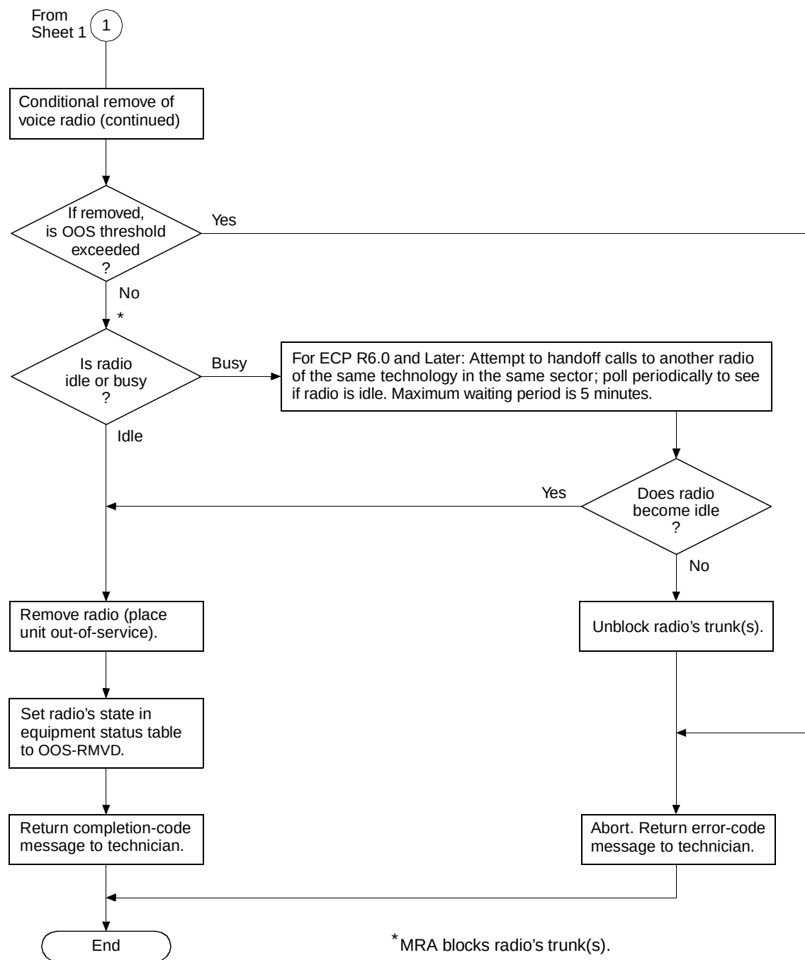
Figure 15-2. Remove Flow of Voice Radio RCU, SBRCU, DRU, or EDRU (Sheet 1 of 3)
