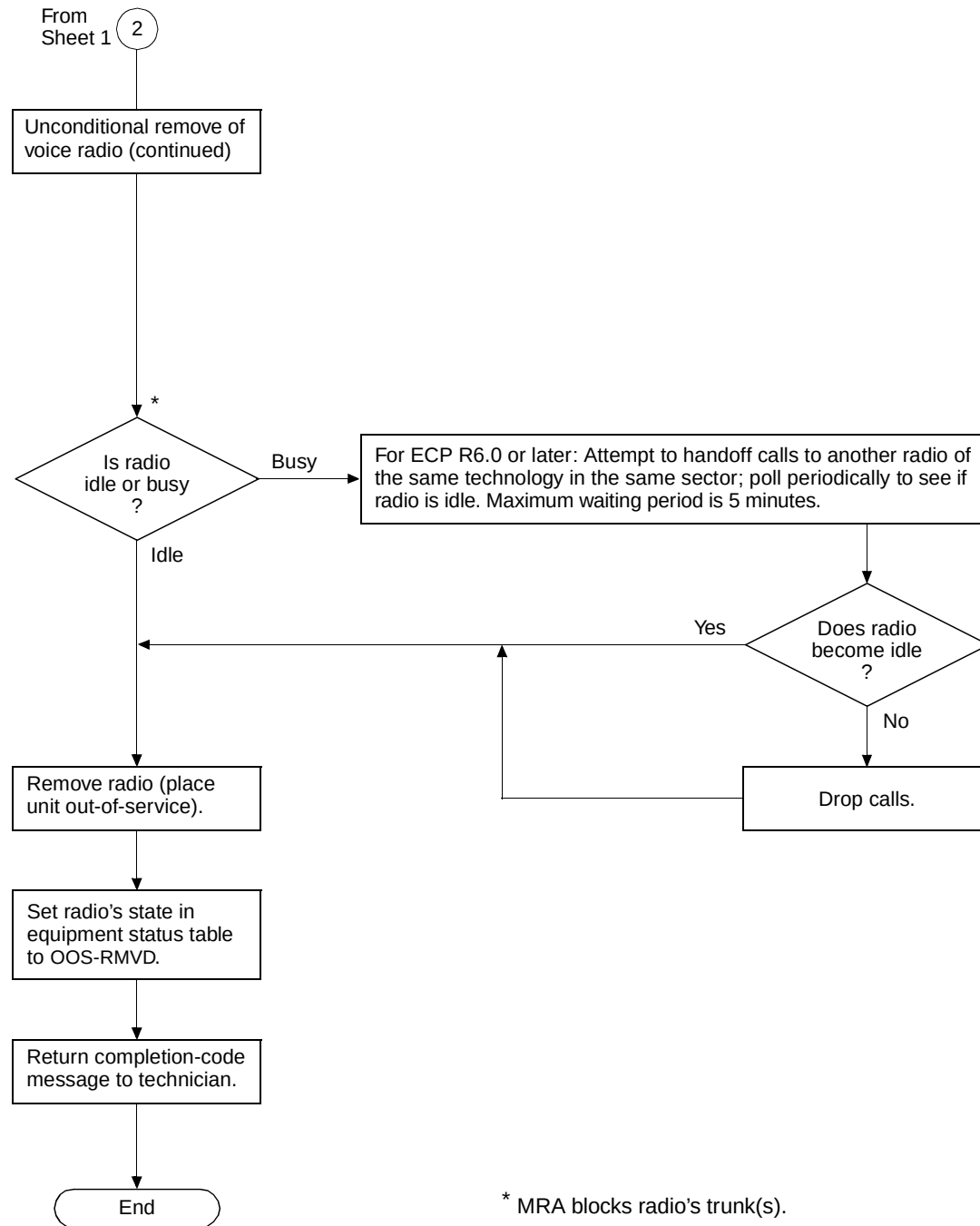
Figure 15-3. Remove Flow of Voice Radio RCU, SBRCU, DRU, or ED RU (Sheet 3 of 3)
