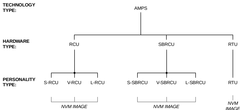
Figure 9-1. AMPS Radio Maintenance Units and Personality Types
