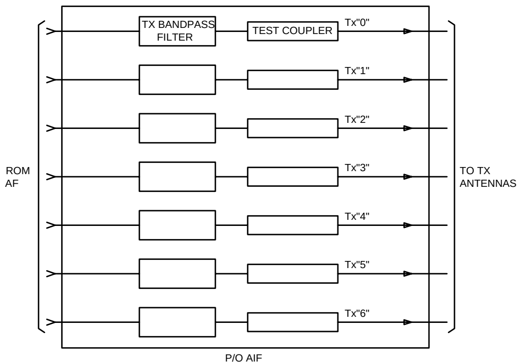
Figure 10-7. Antenna Coupler
