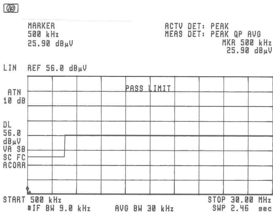
Figure 5.1 Line Conducted
