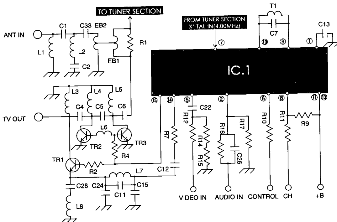
Diagram of IC1 RF converter / switch Type: QAU0115-x
