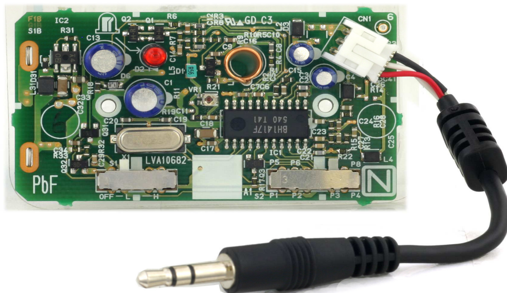
< Topside >
