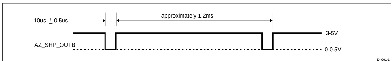
Figure 9. AZ_SHP_OUTB / AZIM_DNEG
