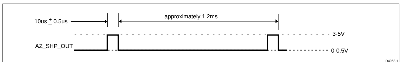
Figure 10. AZ_SHP_OUT / AZIM_DPOS
