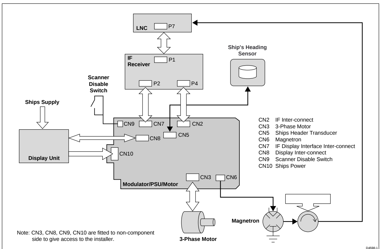
Figure 4. Scanner Interfaces
