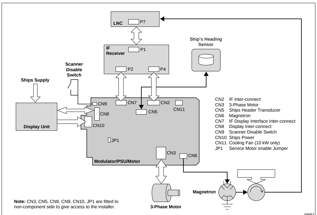
Figure 4. Scanner Interfaces
