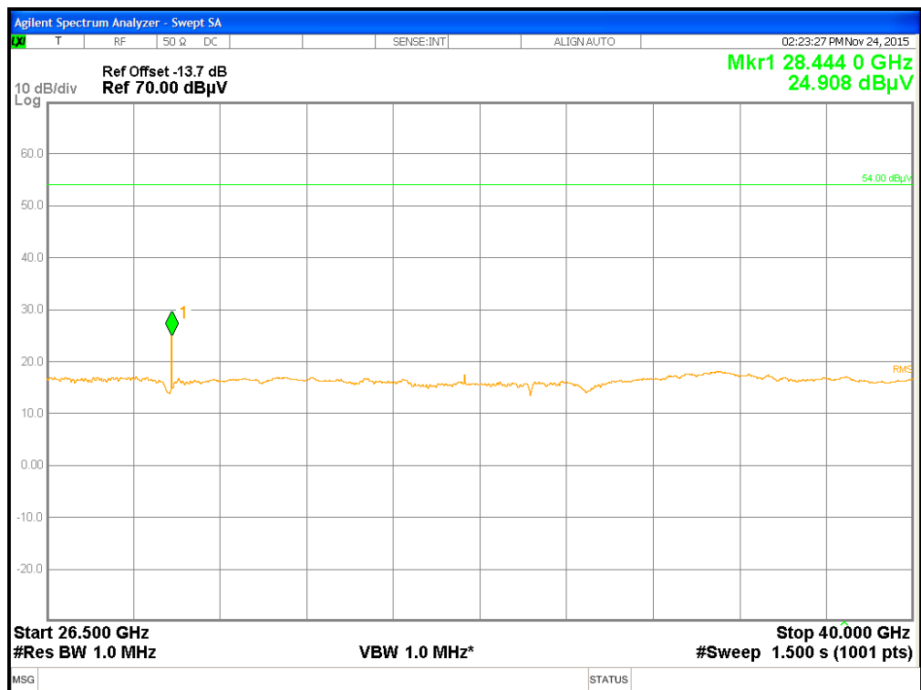
Plot No. 8: 26.5 GHz – 40 GHz
