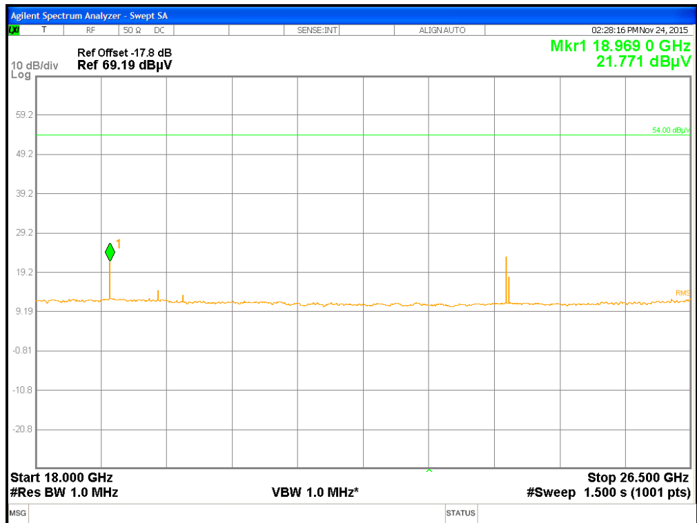
Plot No. 7: 18 – 26.5 GHz
