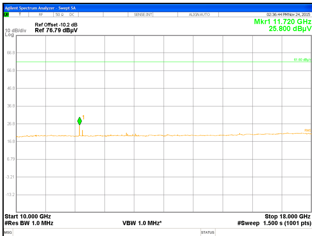
Plot No. 6: 10 – 18 GHz
