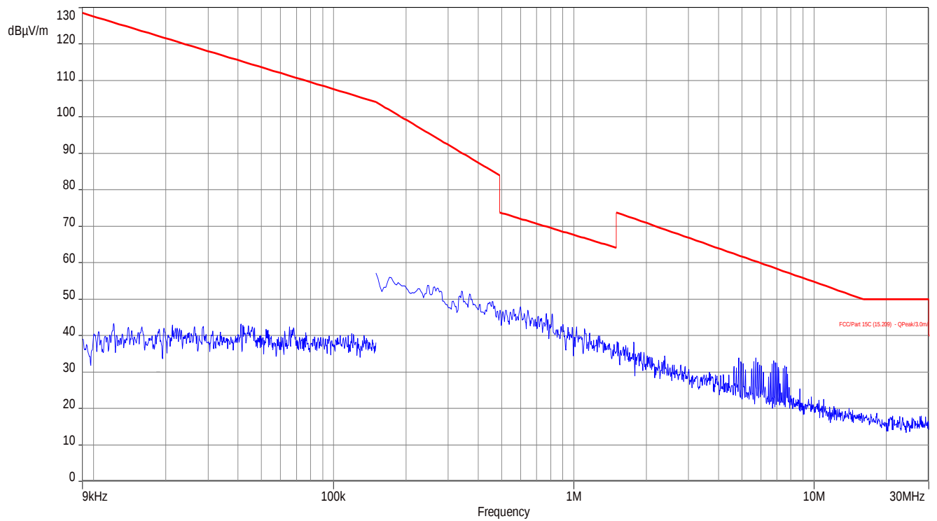
Plot No. 3: magnetic
