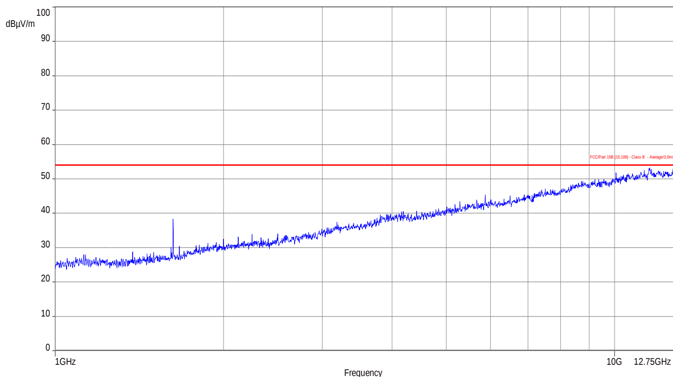
Plot No. 5: 1 GHz – 12.75 GHz
