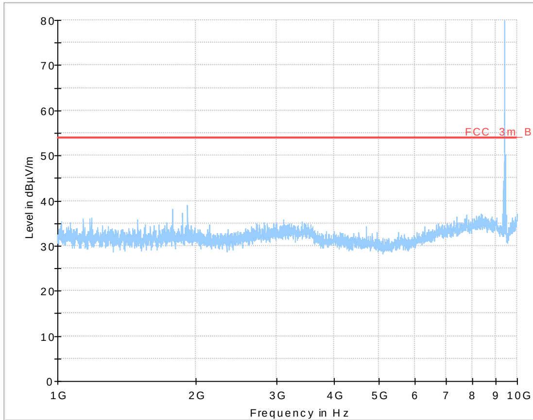
Plot No. 11: Tx on, long pulse
