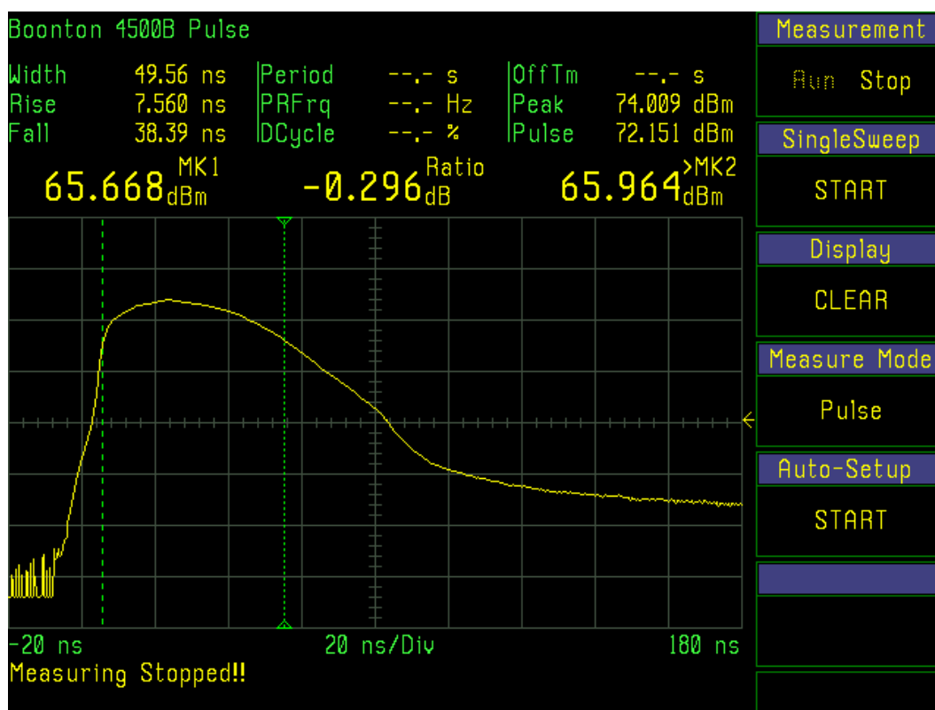
Plot No. 1: EEV Magnetron, Type MG5424, short pulse
