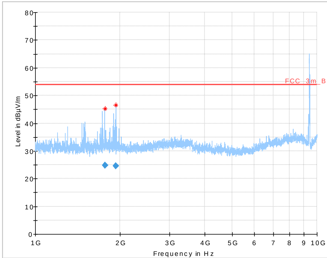
Plot No. 5: Tx on, short pulse
