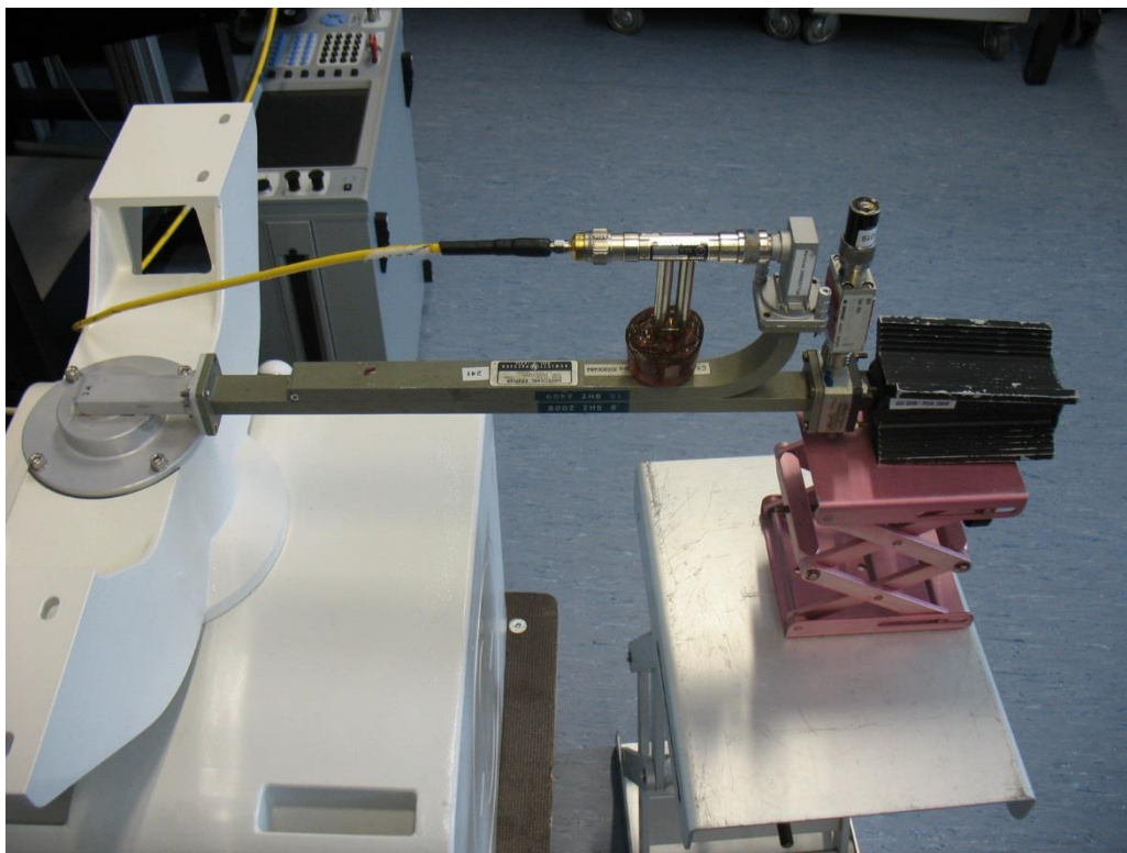
Photo No. 5: conducted measurements up to 15 GHz
