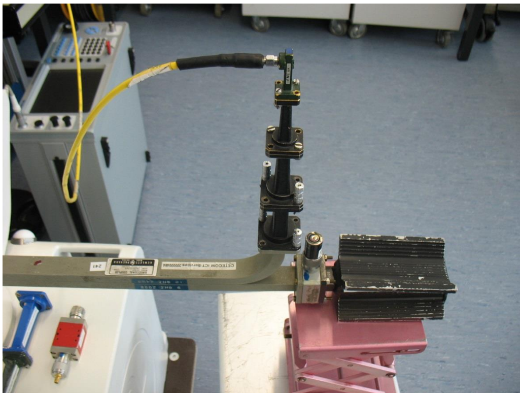
Photo No. 7: measurements up to 40 GHz
