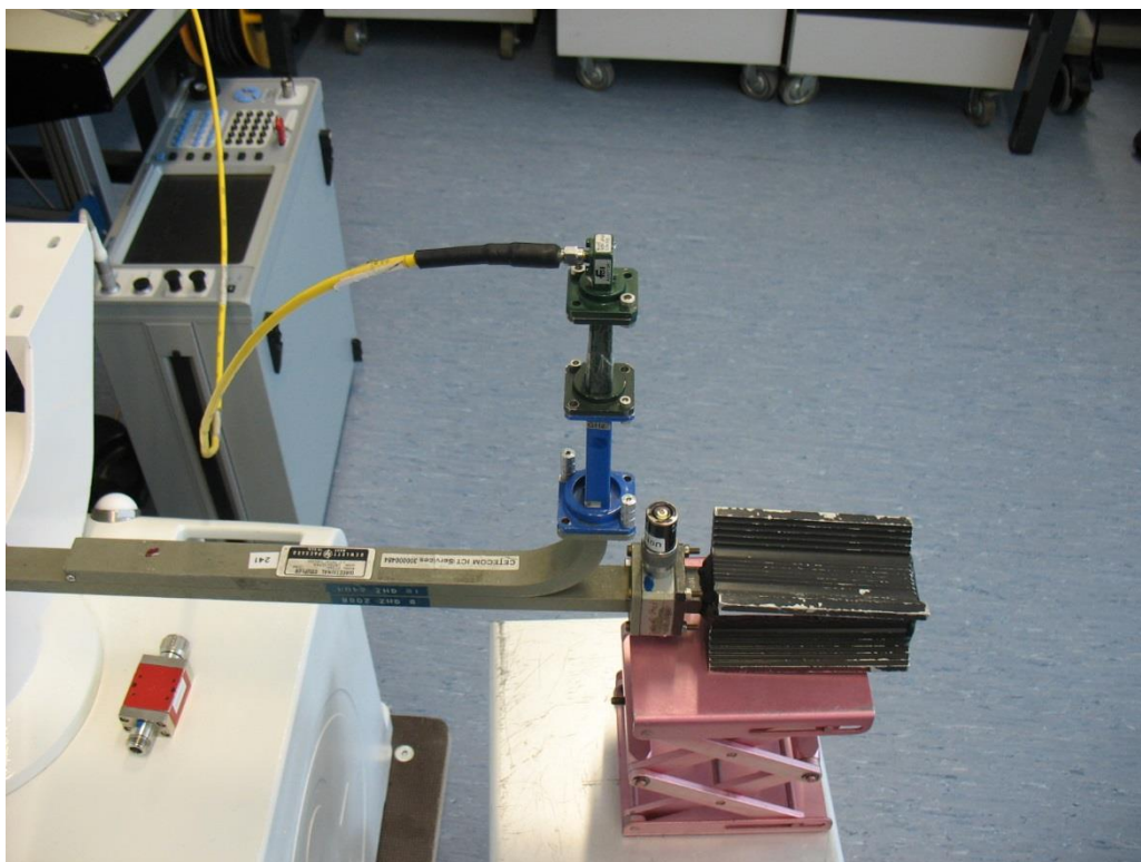
Photo No. 6: measurements up to 26.5 GHz
