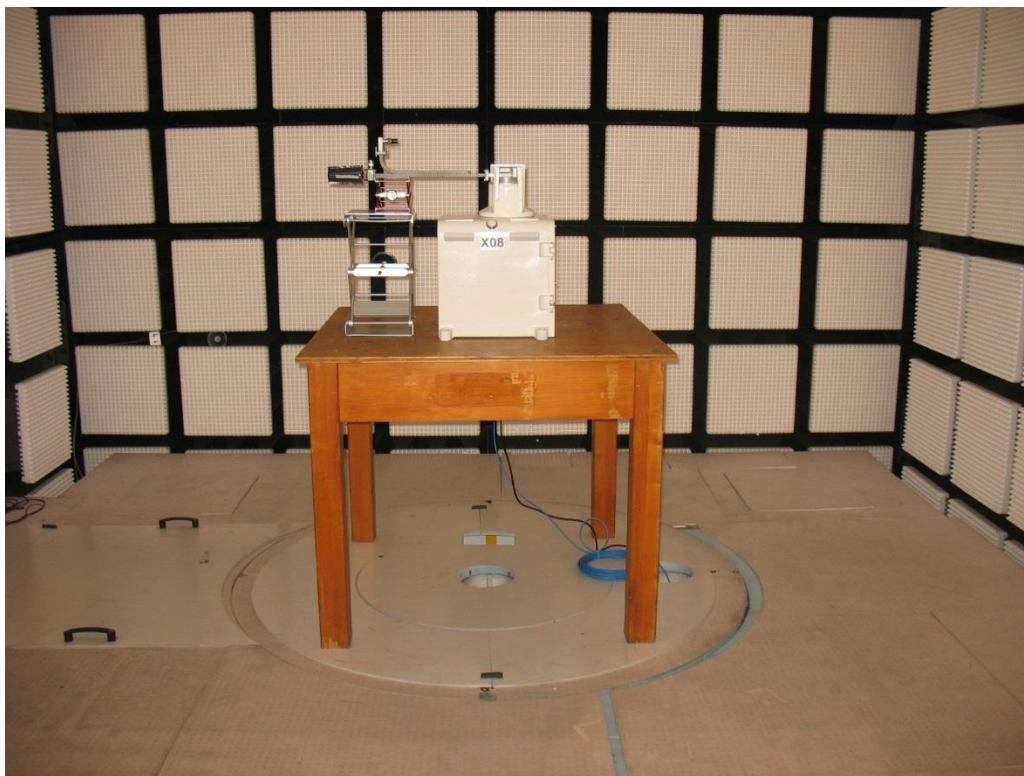
Photo No. 3: radiated spurious
