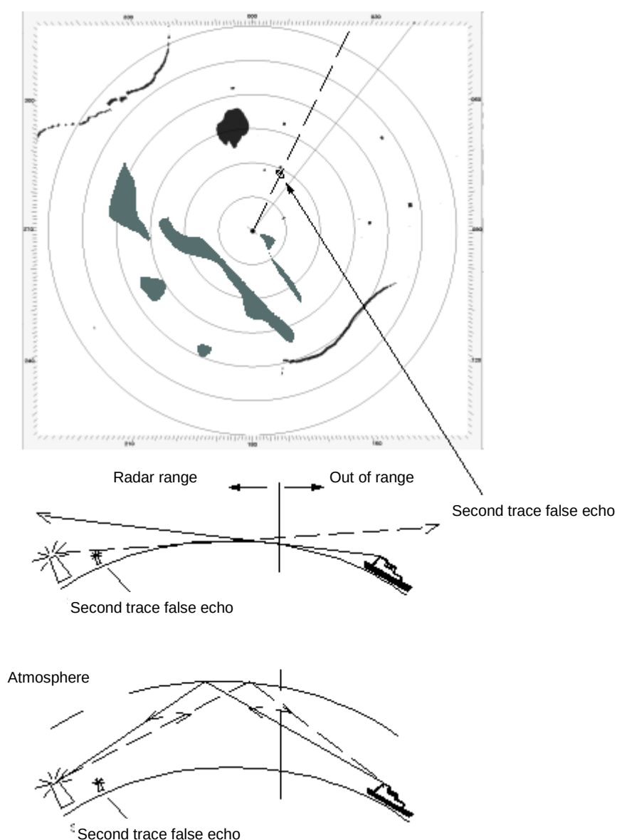
Figure 3-8 Second Trace False Echo, Duct Effect
