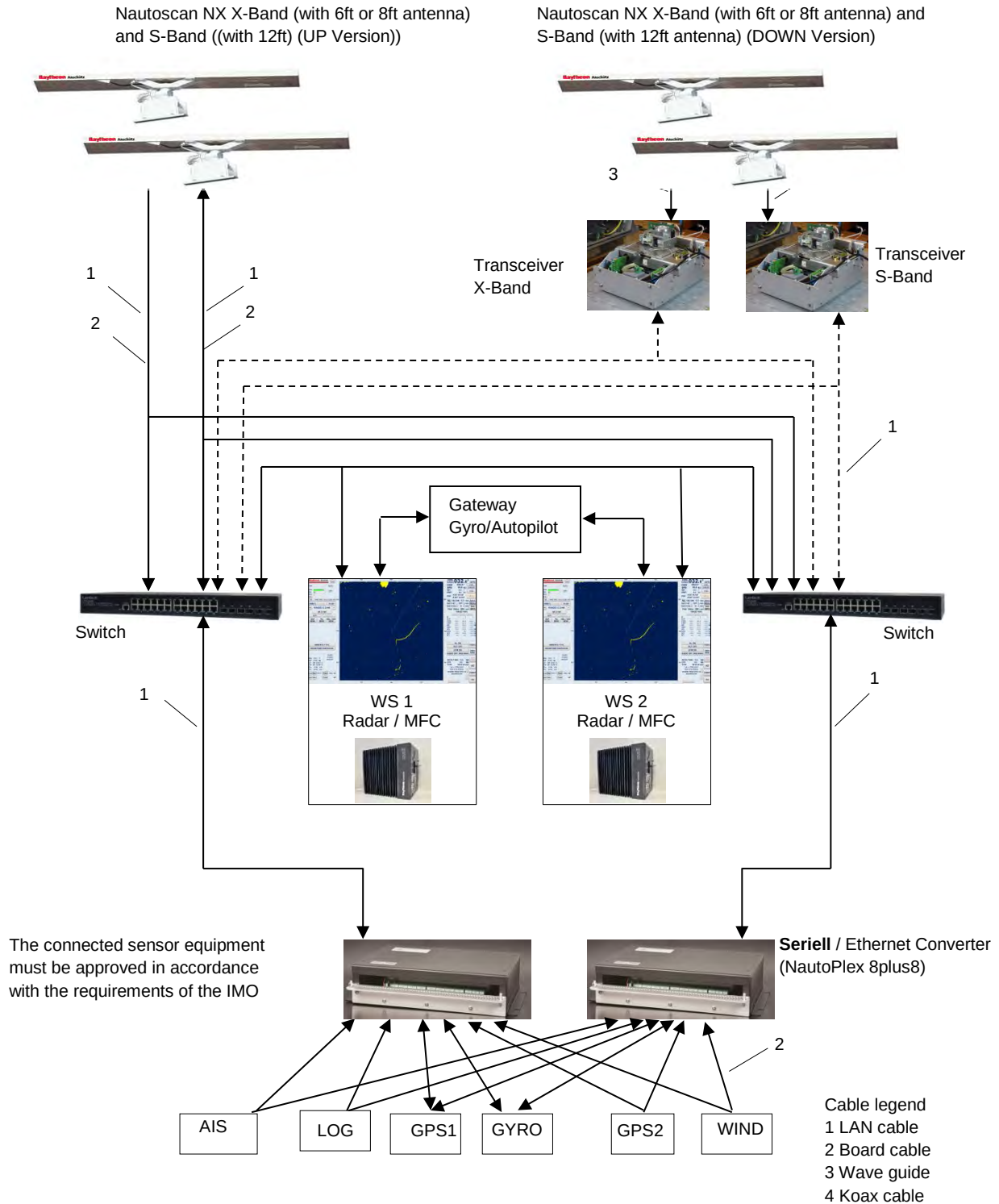
Figure 1-3 Double Radar System
