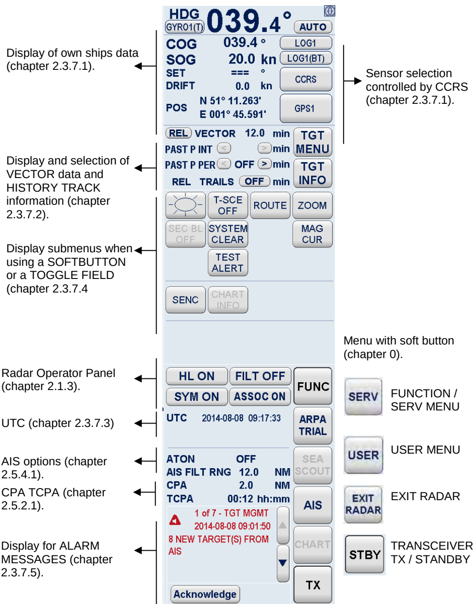
Figure 2-35 Radar Information Panel
