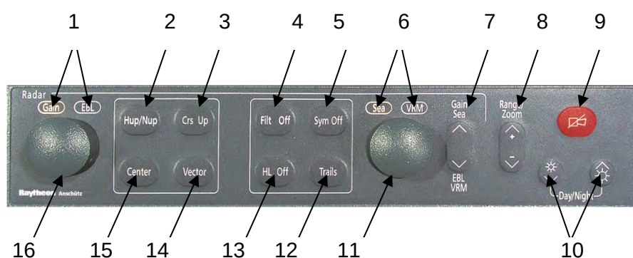
Figure 2-4 Radar Operator Panel
