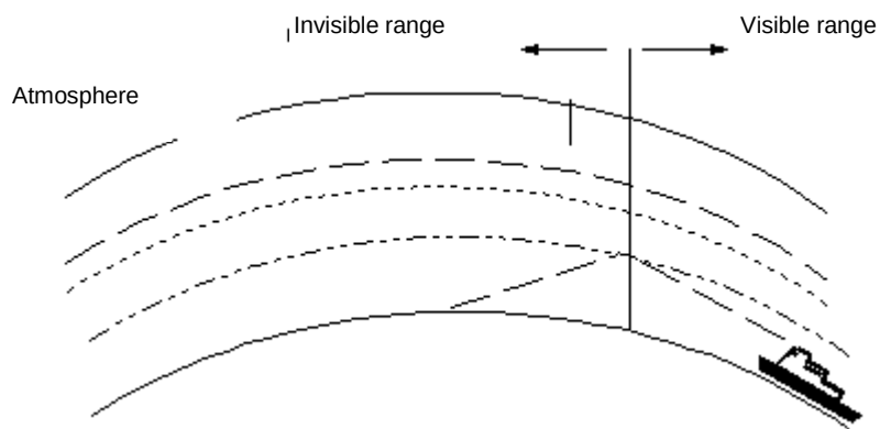
Figure 3-9 Atmospheric Condition
