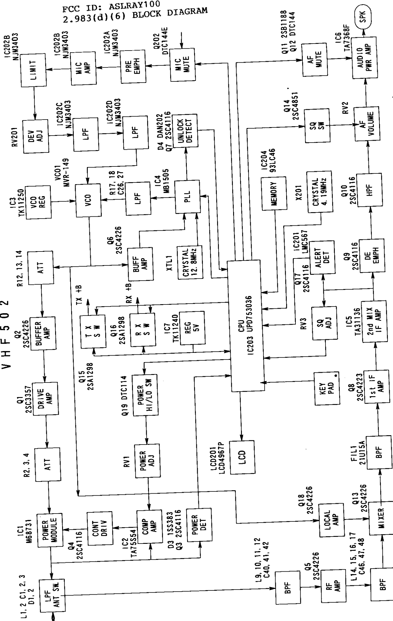
Fig. 4-1 BLOCK DIAGRAM
