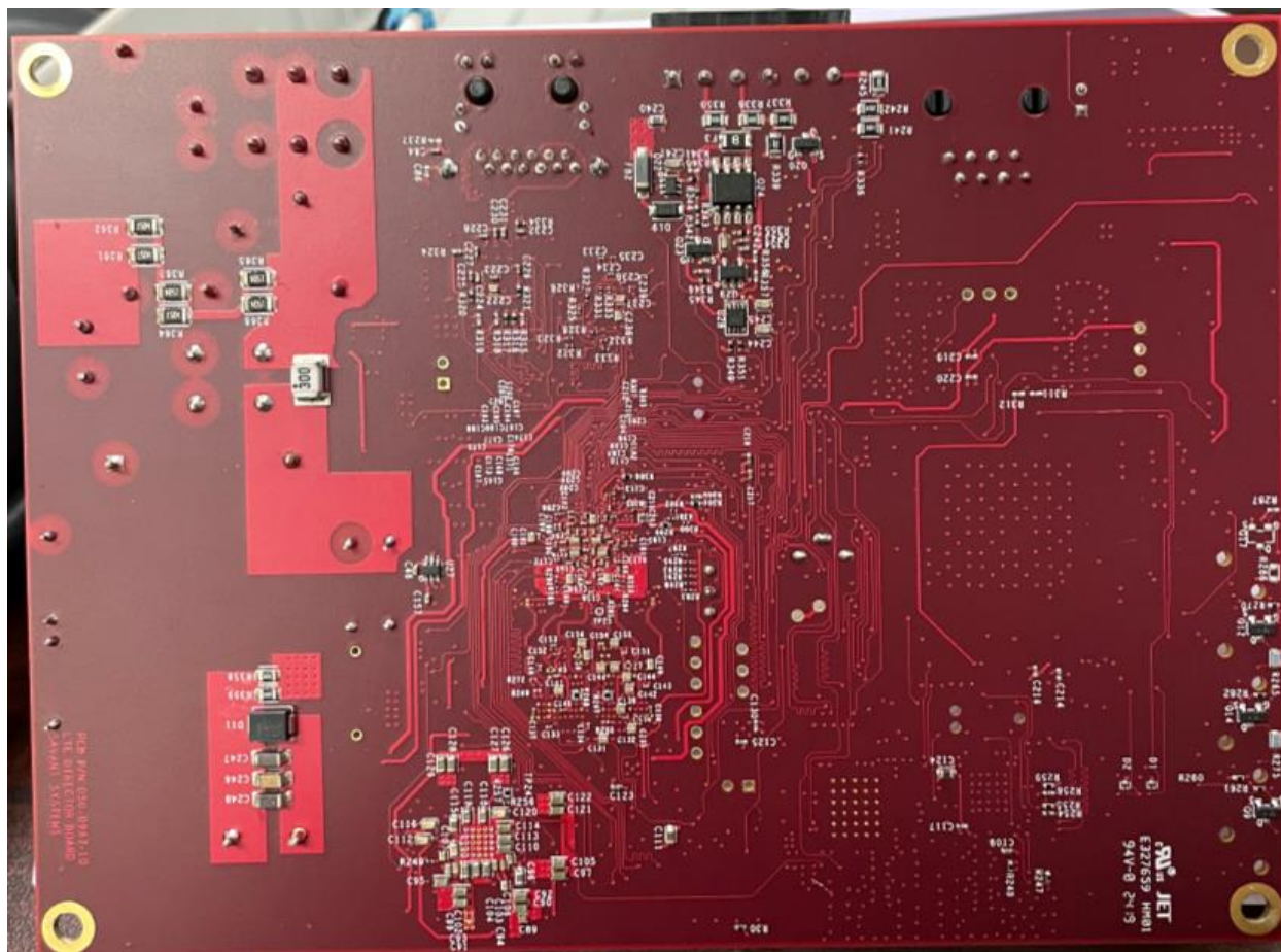
Figure 4: DIRECTOR PCB Back
