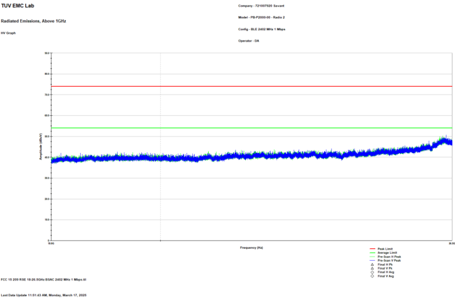
Figure 2.8.7-19: Reference plot for Radiated Spurious Emissions – 18 GHz – 26.5 GHz – LCH – 1 Mbps – Radio 2
