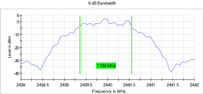
Figure 2.4.7-8: 6 dB BW - MCH – 2 Mbps
