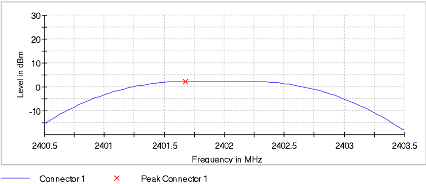
Figure 2.3.7-1: Output Power - LCH – 1 Mbps
