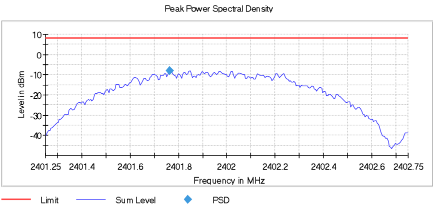
Figure 2.5.6-1: PSD – LCH – 1 Mbps
