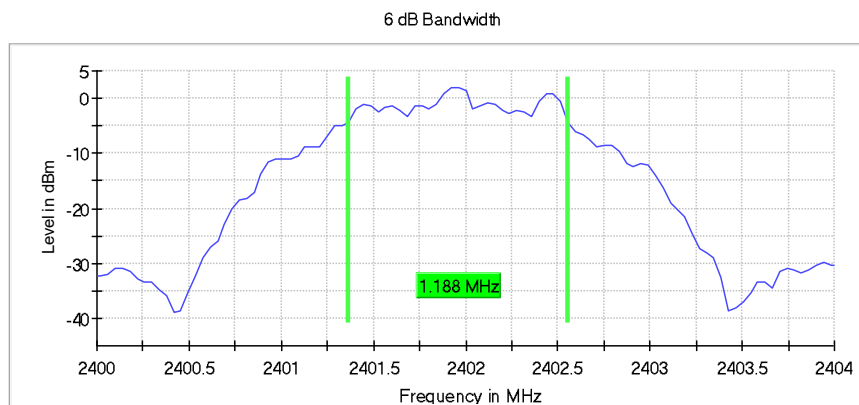
Figure 2.4.7-7: 6 dB BW - LCH – 2 Mbps
