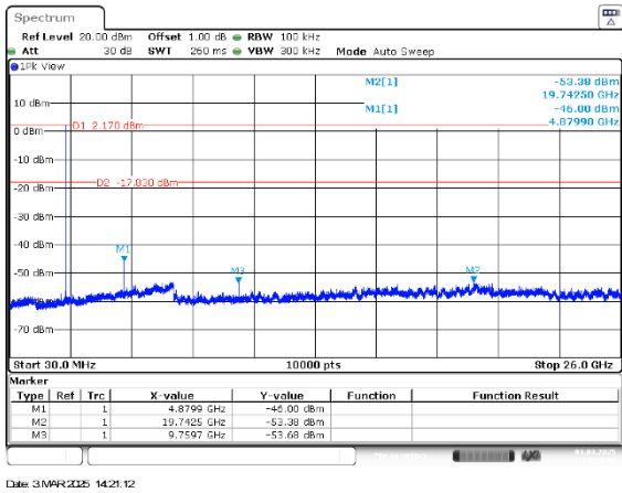
Figure 2.7.7-2: 30MHz – 26GHz – MCH – 1 Mbps
