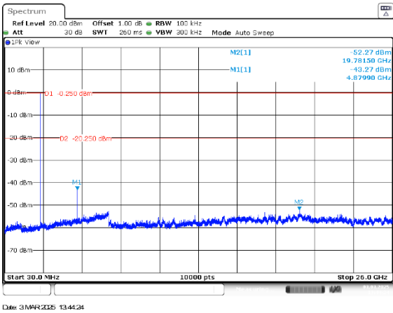
Figure 2.7.6-5: 30MHz – 26GHz – MCH – 2 Mbps
