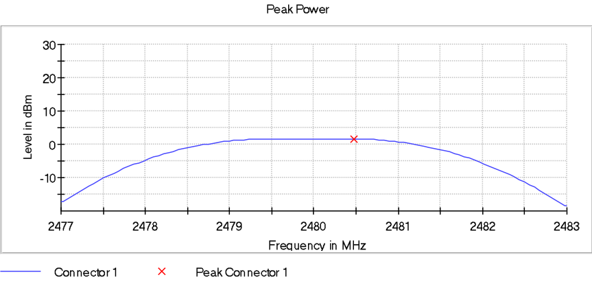
Figure 2.3.6-6: Output Power - HCH - 2 Mbps
