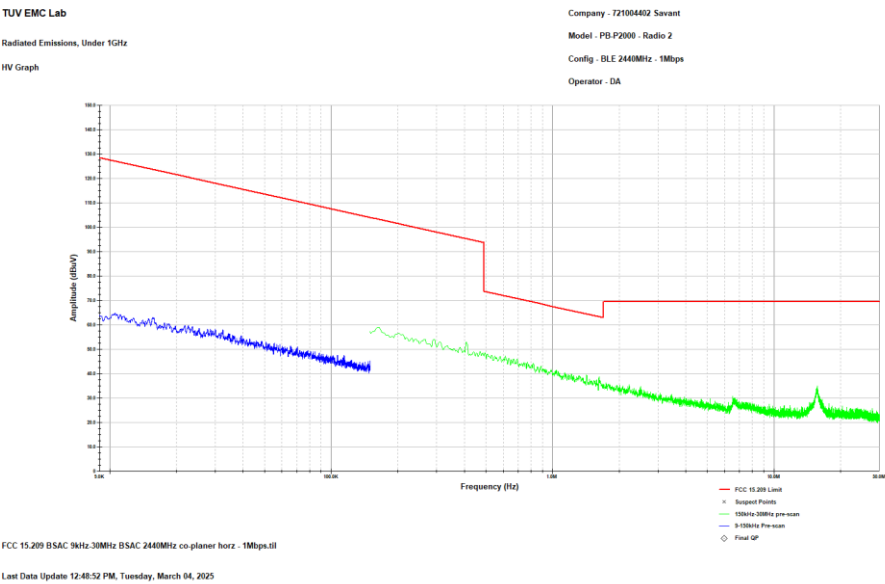
Figure 2.8.7-14: Reference plot for Radiated Spurious Emissions– 9 kHz – 30 MHz – Co-Planar Horz. - MCH - 1 Mbps – Radio 2
