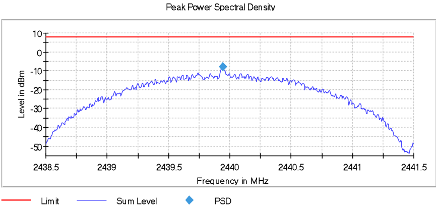
Figure 2.5.7-5: PSD – MCH – 2 Mbps
