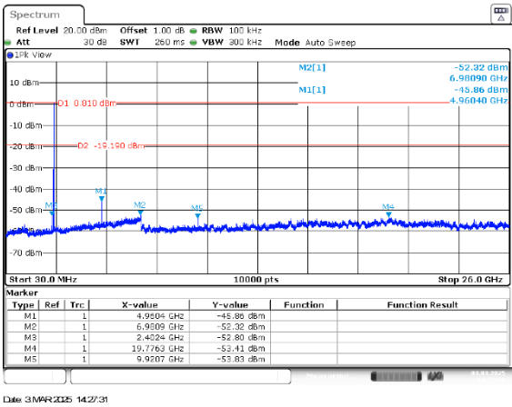
Figure 2.7.7-3: 30MHz – 26GHz – HCH – 1 Mbps
