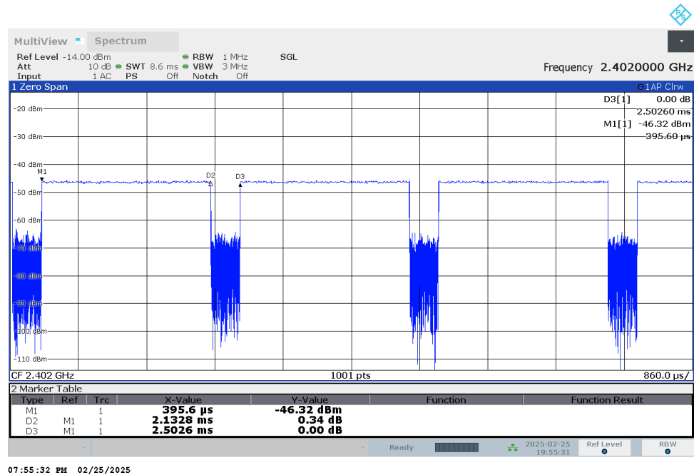
Figure 2.8.6-1: Duty Cycle
