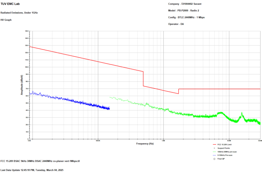
Figure 2.8.7-15: Reference plot for Radiated Spurious Emissions– 9 kHz – 30 MHz – Co-Planar Vert. - MCH - 1 Mbps – Radio 2
