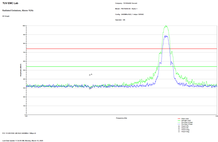
Figure 2.8.6-2: Reference Plot for Radiated Lower Band-edge – LCH – 1 Mbps – Radio 1
