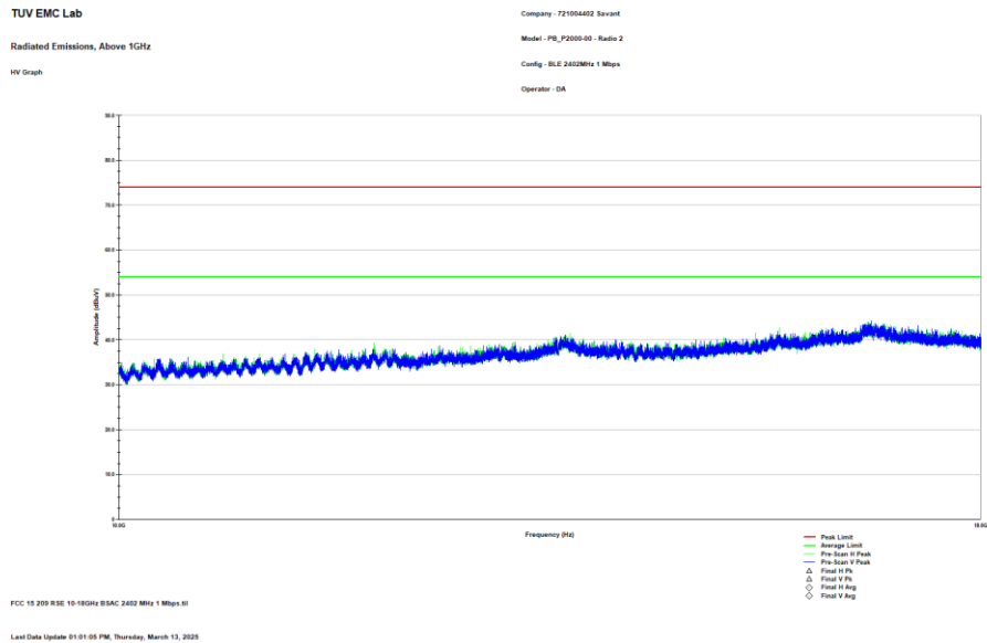
Figure 2.8.7-18: Reference plot for Radiated Spurious Emissions – 10 GHz – 18 GHz – LCH – 1 Mbps – Radio 2
