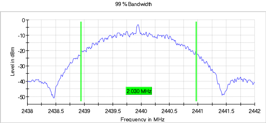
Figure 2.4.7-11: 99% BW - MCH – 2 Mbps
