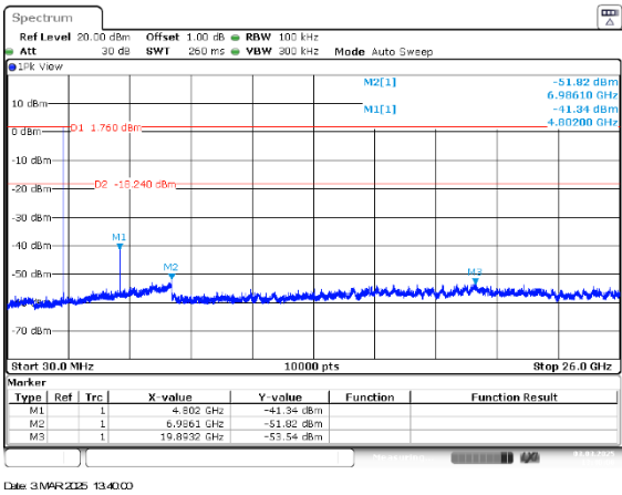
Figure 2.7.6-4: 30MHz – 26GHz – LCH – 2 Mbps
