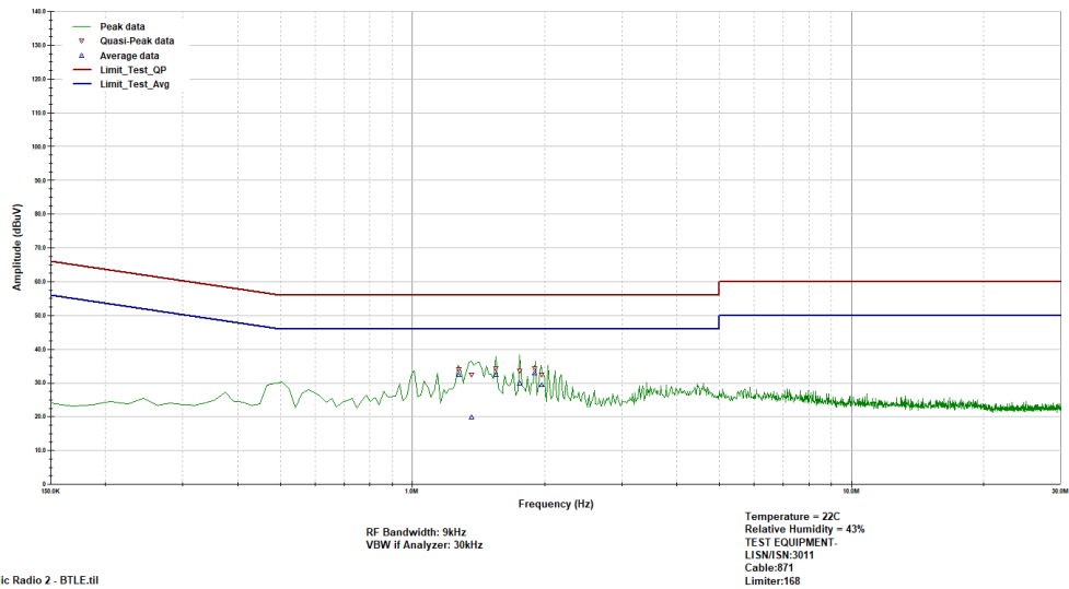
Figure 2.2.7-1: Conducted Emission Plot – Line 1
