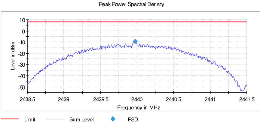
Figure 2.5.6-5: PSD – MCH – 2 Mbps
