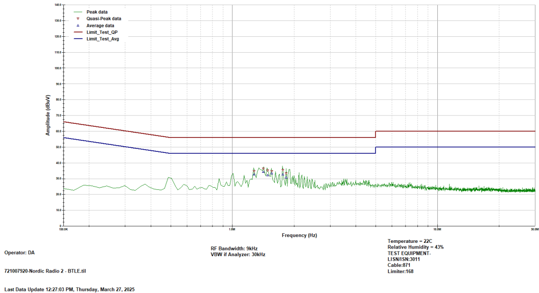
Figure 2.2.7-2: Conducted Emission Plot – Nuetral
