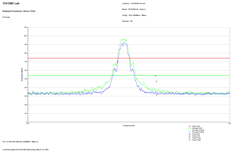
Figure 2.8.7-12: Reference Plot for Radiated Upper Band-edge – HCH – 1 Mbps – Radio 2
