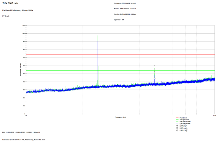
Figure 2.8.7-17: Reference plot for Radiated Spurious Emissions – 1 GHz – 10 GHz – LCH – 1 Mbps – Radio 2 Note: The emission above the limit line is the Fundamental Frequency.
