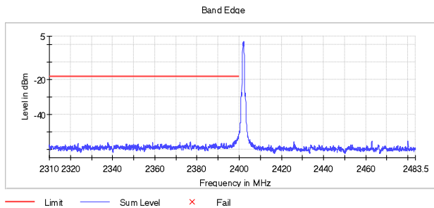
Figure 2.6.6-1: Lower Band-edge – 1Mbps
