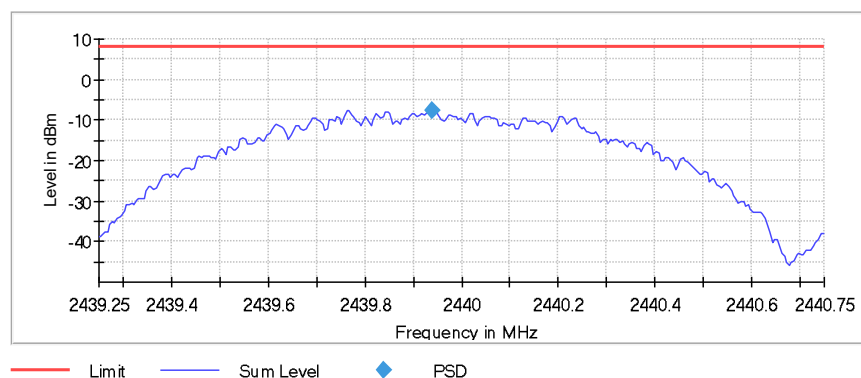
Figure 2.5.7-2: PSD – MCH – 1 Mbps
