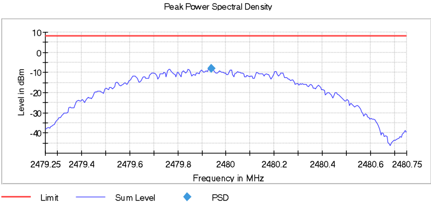
Figure 2.5.7-3: PSD – HCH – 1 Mbps
