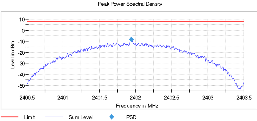
Figure 2.5.7-4: PSD – LCH – 2 Mbps
