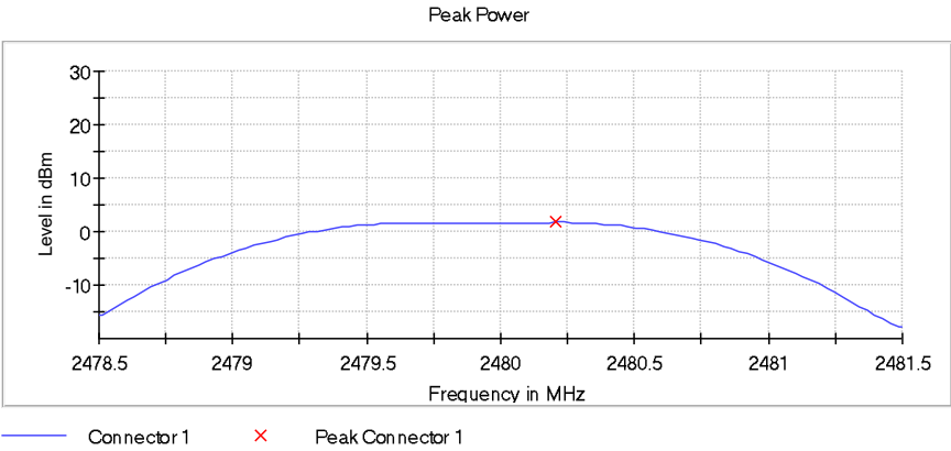
Figure 2.3.7-3: Output Power - HCH - 1 Mbps
