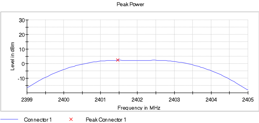
Figure 2.3.7-4: Output Power - LCH – 2 Mbps
