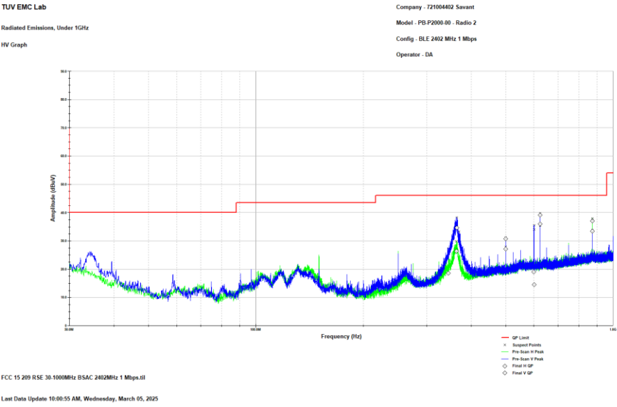
Figure 2.8.7-16: Reference plot for Radiated Spurious Emissions – 30 MHz – 1 GHz – LCH – 1 Mbps – Radio 2
