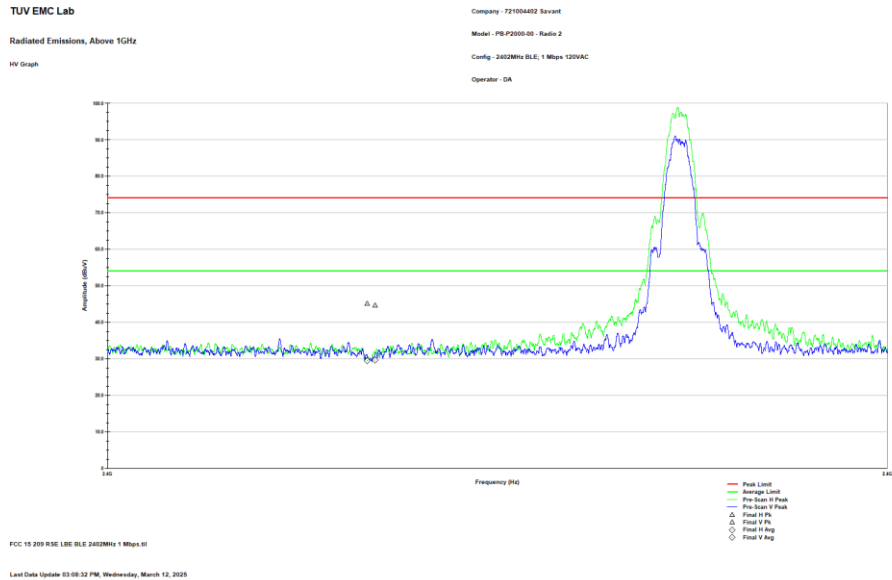
Figure 2.8.7-11: Reference Plot for Radiated Lower Band-edge – LCH – 1 Mbps – Radio 2
