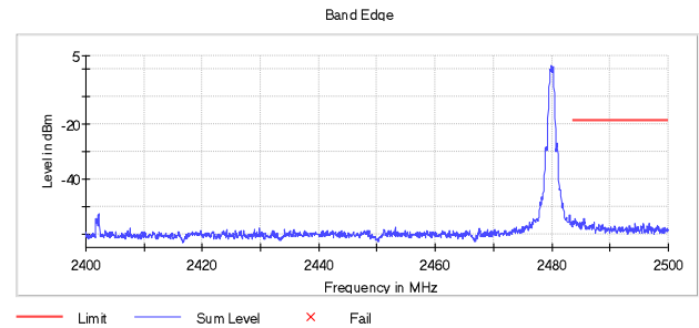
Figure 2.6.7-2: Upper Band-edge – 1Mbps
