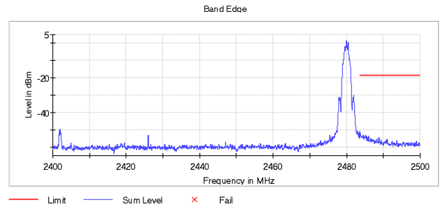
Figure 2.6.7-4: Upper Band-edge – 2 Mbps
