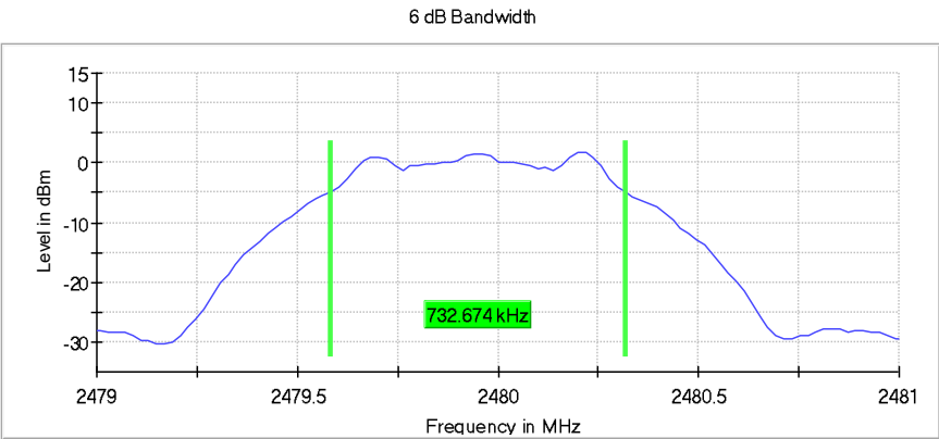
Figure 2.4.7-3: 6 dB BW - HCH – 1 Mbps
