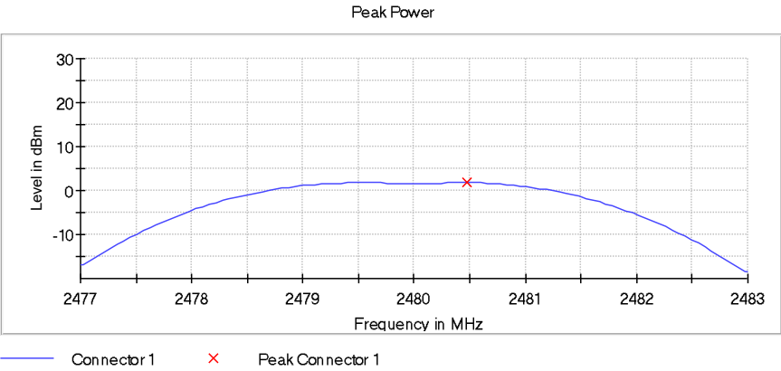
Figure 2.3.7-6: Output Power - HCH - 2 Mbps
