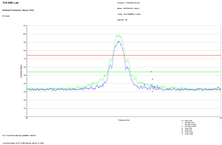
Figure 2.8.6-3: Reference Plot for Radiated Upper Band-edge – HCH – 1 Mbps – Radio 1
