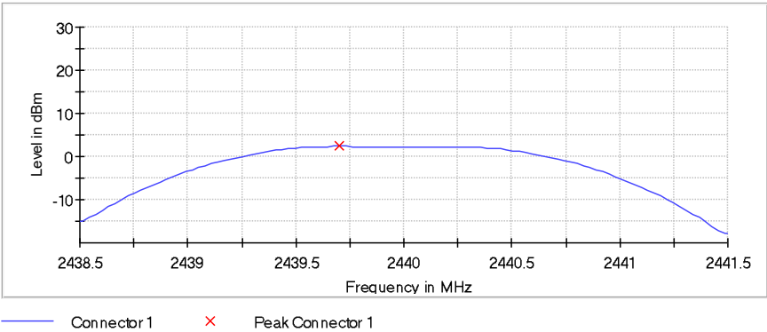
Figure 2.3.7-2: Output Power - MCH – 1 Mbps
