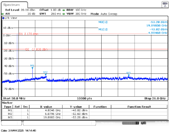
Figure 2.7.7-1: 30MHz – 26GHz – LCH – 1 Mbps
