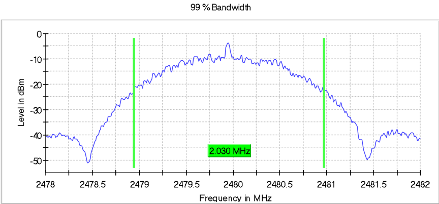
Figure 2.4.7-12: 99% BW - HCH – 2 Mbps
