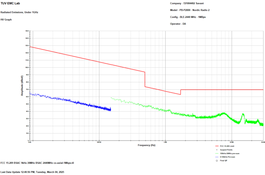
Figure 2.8.7-13: Reference plot for Radiated Spurious Emissions – 9 kHz – 30 MHz – Co-Axial - MCH - 1 Mbps – Radio 2
