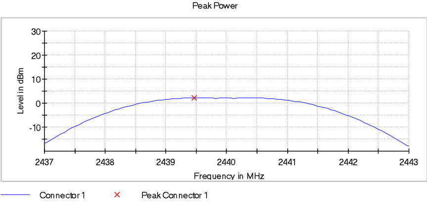
Figure 2.3.6-5: Output Power - MCH – 2 Mbps
