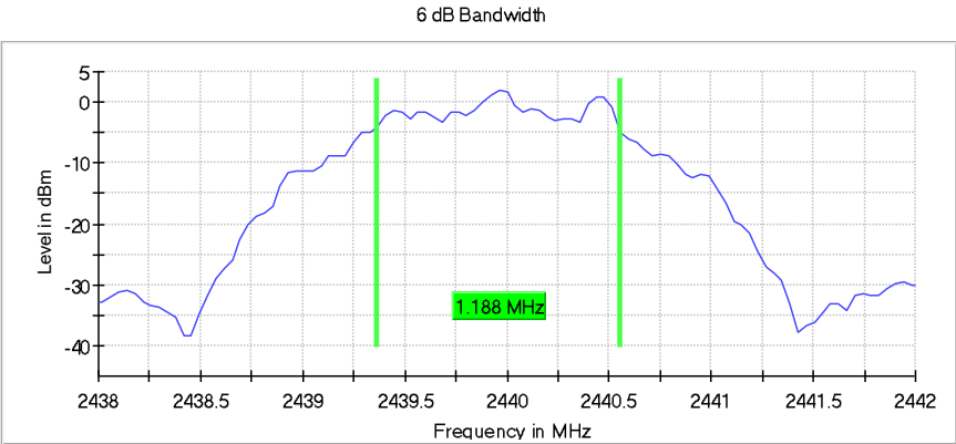
Figure 2.4.6-8: 6 dB BW - MCH – 2 Mbps
