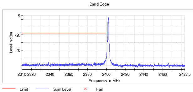
Figure 2.6.7-1: Lower Band-edge – 1Mbps
