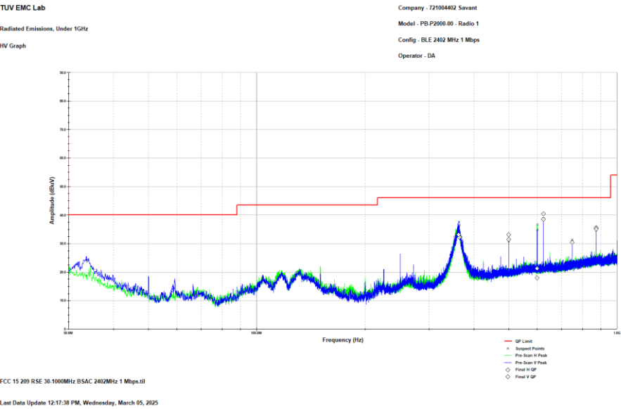
Figure 2.8.6-7: Reference plot for Radiated Spurious Emissions – 30 MHz – 1 GHz – LCH – 1 Mbps – Radio 1
