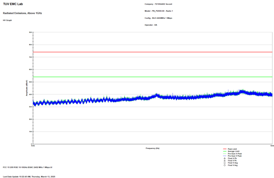
Figure 2.8.6-9: Reference plot for Radiated Spurious Emissions – 10 GHz – 18 GHz – LCH – 1 Mbps – Radio 1
