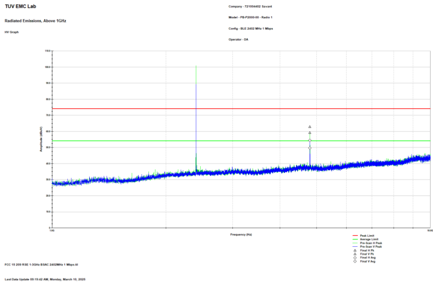
Figure 2.8.6-8: Reference plot for Radiated Spurious Emissions – 1 GHz – 10 GHz – LCH – 1 Mbps – Radio 1 Note: The emission above the limit line is the Fundamental Frequency.
