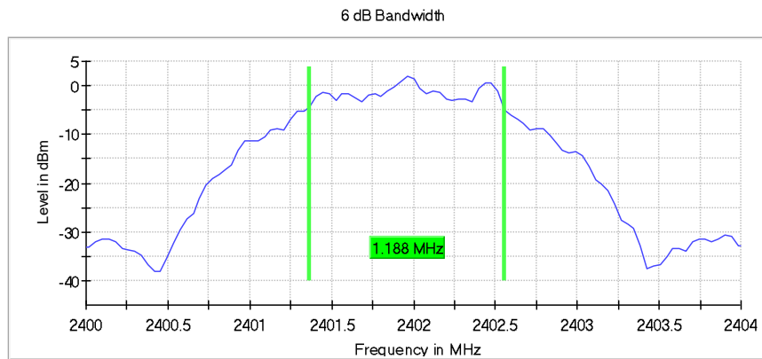
Figure 2.4.6-7: 6 dB BW - LCH – 2 Mbps
