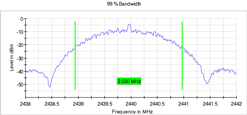
Figure 2.4.6-11: 99% BW - MCH – 2 Mbps
