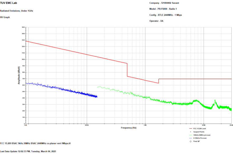
Figure 2.8.6-6: Reference plot for Radiated Spurious Emissions– 9 kHz – 30 MHz – Co-Planar Vert. - MCH - 1 Mbps – Radio 1
