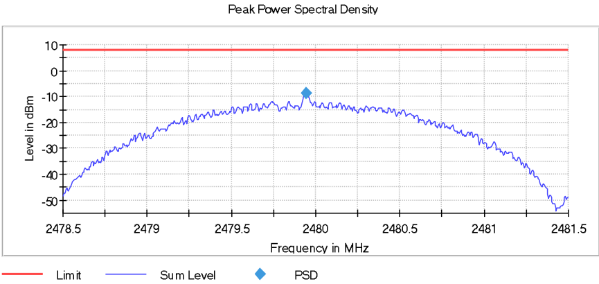
Figure 2.5.7-6: PSD – HCH – 2 Mbps
