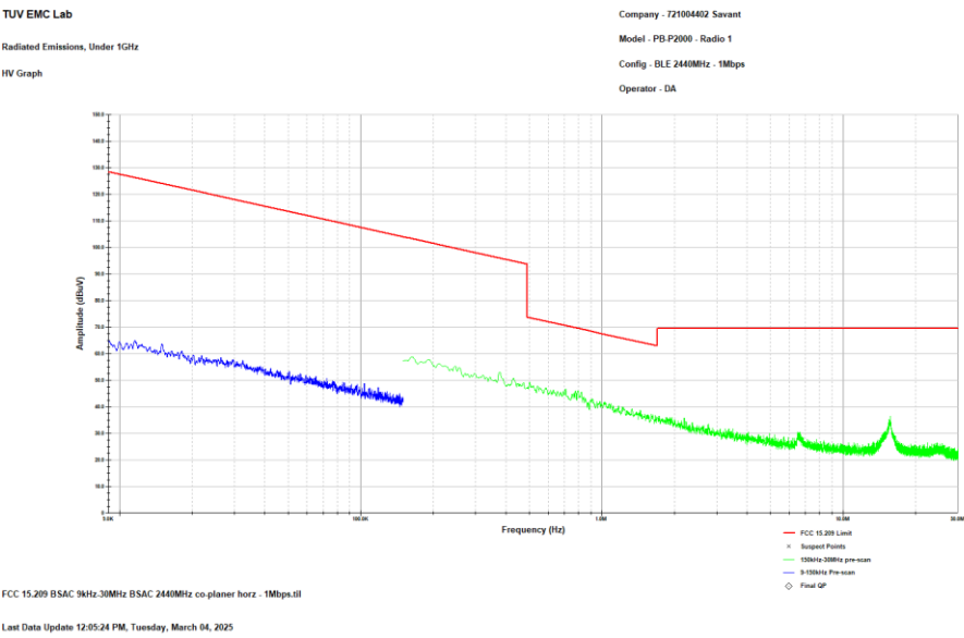
Figure 2.8.6-5: Reference plot for Radiated Spurious Emissions– 9 kHz – 30 MHz – Co-Planar Horz. - MCH - 1 Mbps – Radio 1
