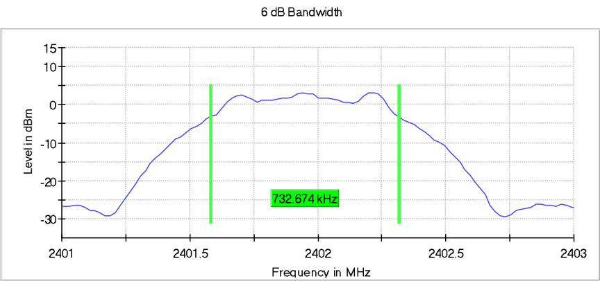
Figure 2.4.7-1: 6 dB BW - LCH – 1 Mbps
