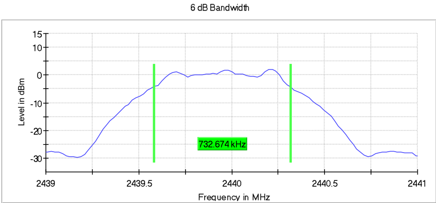
Figure 2.4.6-2: 6 dB BW - MCH – 1 Mbps
