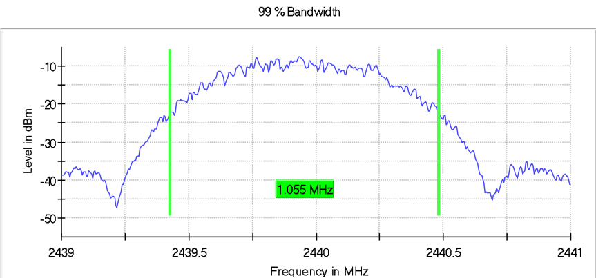
Figure 2.4.7-5: 99% BW - MCH – 1 Mbps
