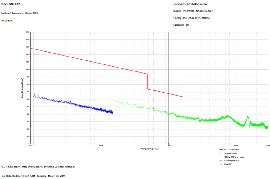
Figure 2.8.6-4: Reference plot for Radiated Spurious Emissions – 9 kHz – 30 MHz – Co-Axial - MCH - 1 Mbps – Radio 1
