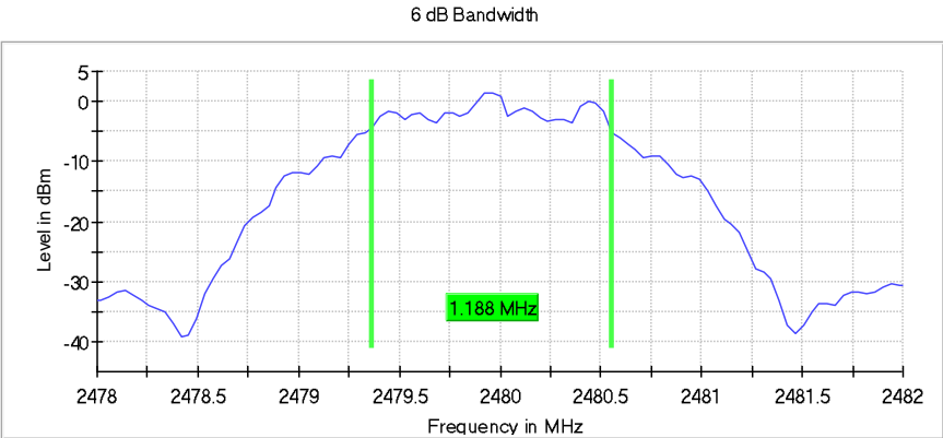
Figure 2.4.7-9: 6 dB BW - HCH – 2 Mbps
