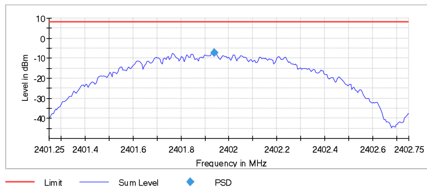
Figure 2.5.7-1: PSD – LCH – 1 Mbps
