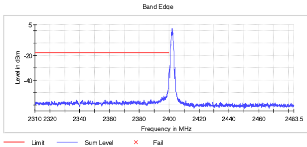
Figure 2.6.7-3: Lower Band-edge – 2 Mbps
