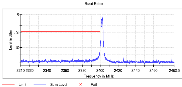
Figure 2.6.6-3: Lower Band-edge – 2 Mbps
