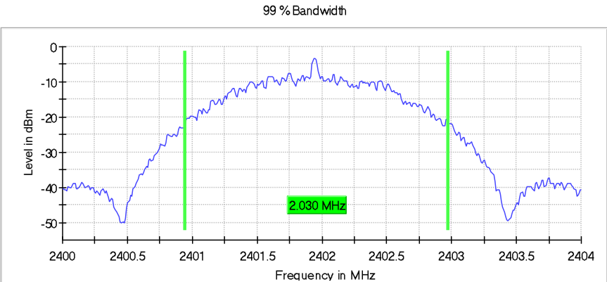
Figure 2.4.7-10: 99% BW - LCH - 2 Mbps
