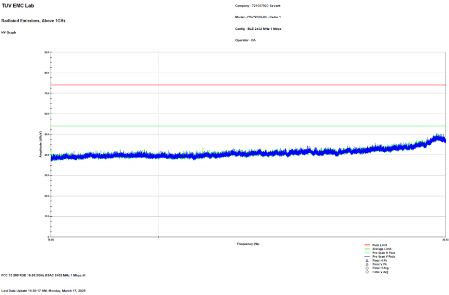
Figure 2.8.6-10: Reference plot for Radiated Spurious Emissions – 18 GHz – 26.5 GHz – LCH – 1 Mbps – Radio 1
