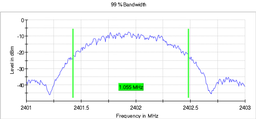
Figure 2.4.7-4: 99% BW - LCH - 1 Mbps
