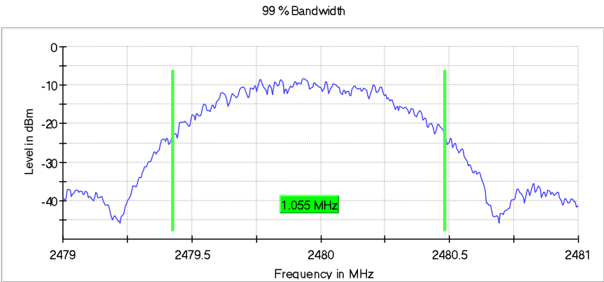
Figure 2.4.7-6: 99% BW - HCH – 1 Mbps
