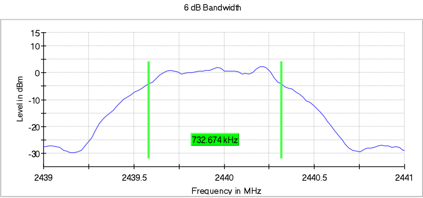
Figure 2.4.7-2: 6 dB BW - MCH – 1 Mbps
