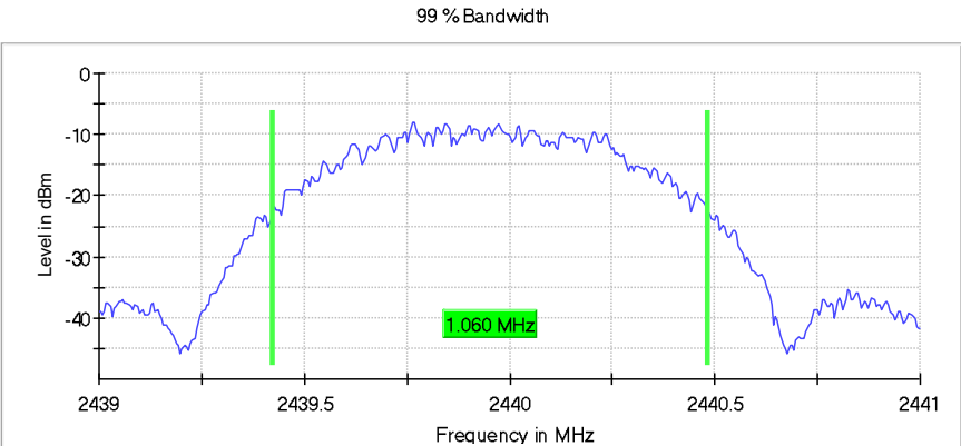
Figure 2.4.6-5: 99% BW - MCH – 1 Mbps
