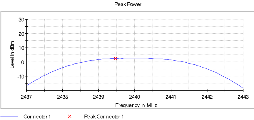
Figure 2.3.7-5: Output Power - MCH – 2 Mbps
