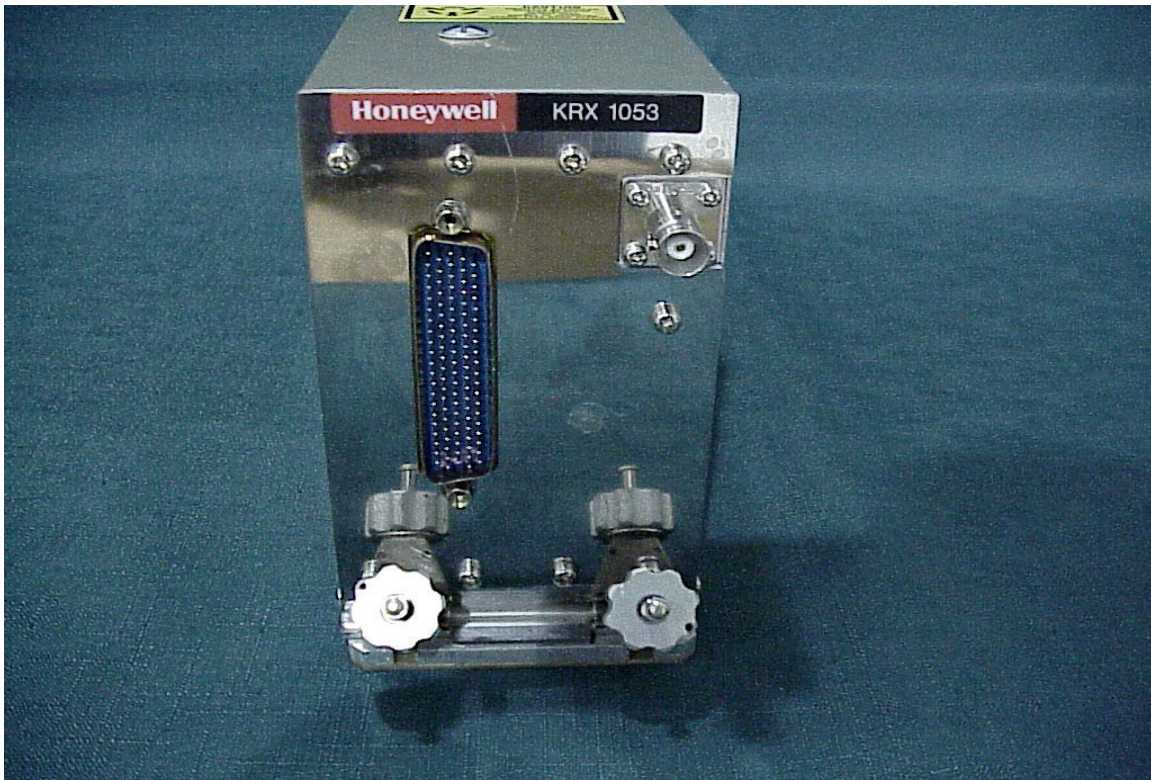
KRX 1053 Receiver Exciter (front view)
