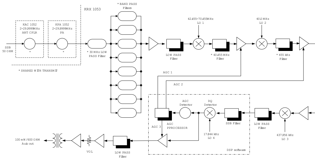
Figure 1-9 CW Receive Mode Block Diagram
