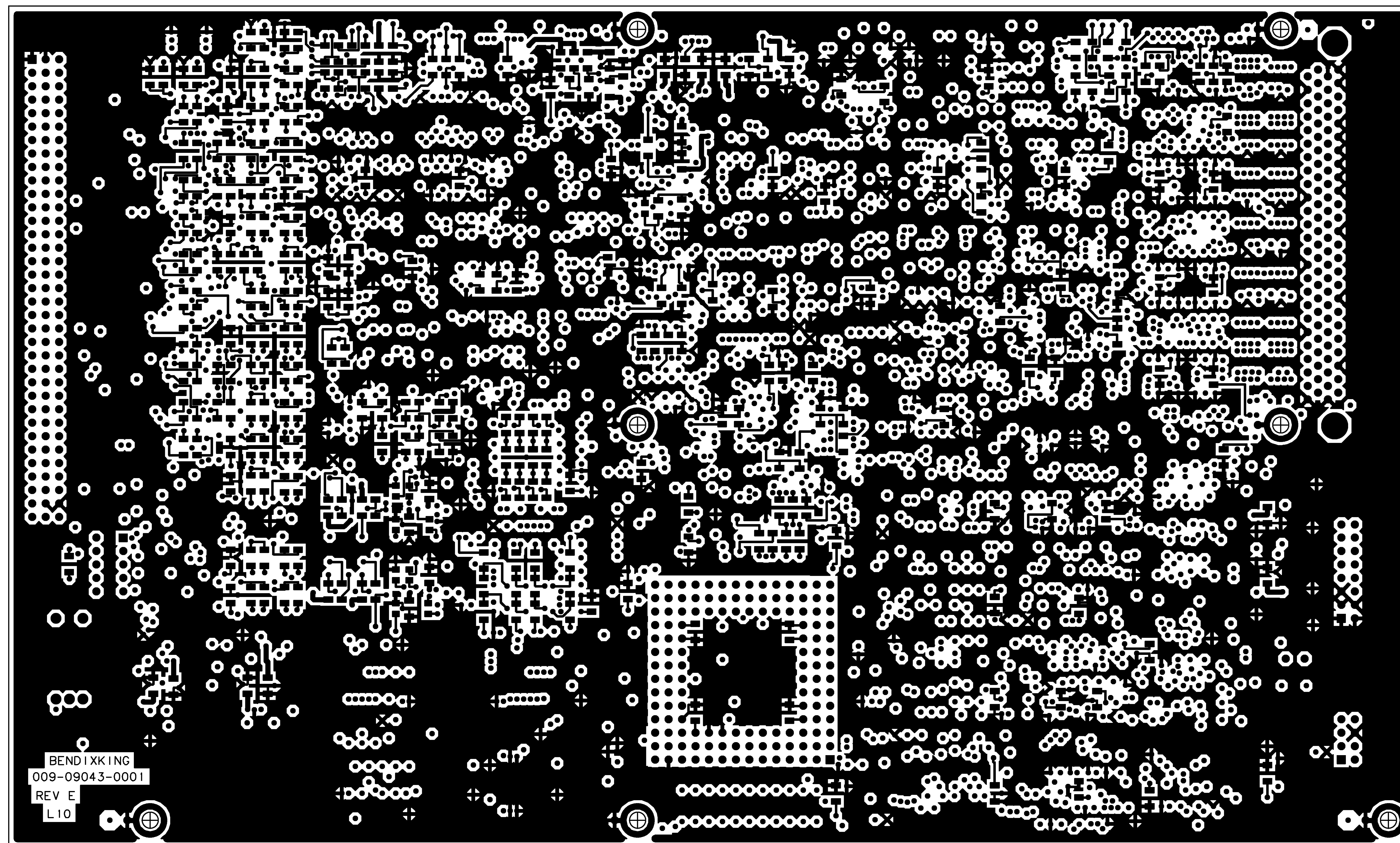
FARSIDE VIEW OF PC BOARD
