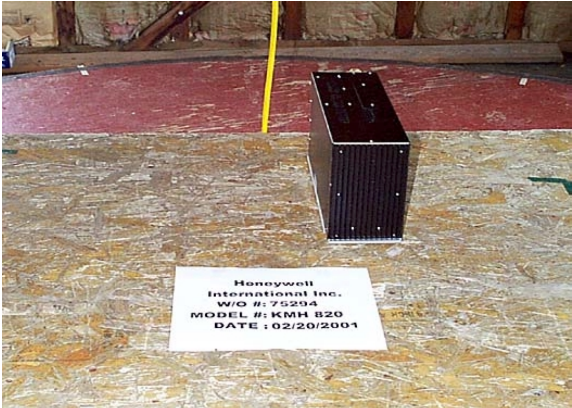
Radiated testing back
