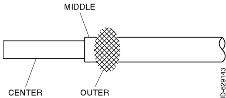
Figure 2-5 (Sheet 1 of 1) Quadraxial Cable Preparation
