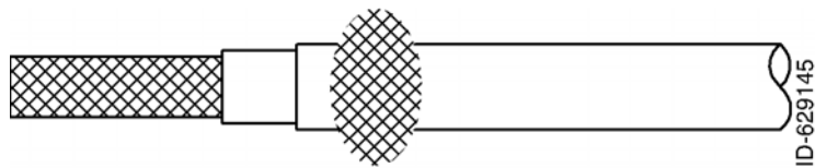
Figure 2-7 (Sheet 1 of 1) Quadrxial Cable Preparation
