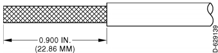
Figure 2-1 (Sheet 1 of 1) Quadraaxial Cable Preparation
