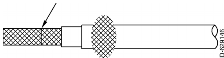
Figure 2-8 (Sheet 1 of 1) Quadrxial Cable Preparation
