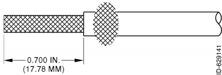
Figure 2-3 (Sheet 1 of 1) Quadraxial Cable Preparation
