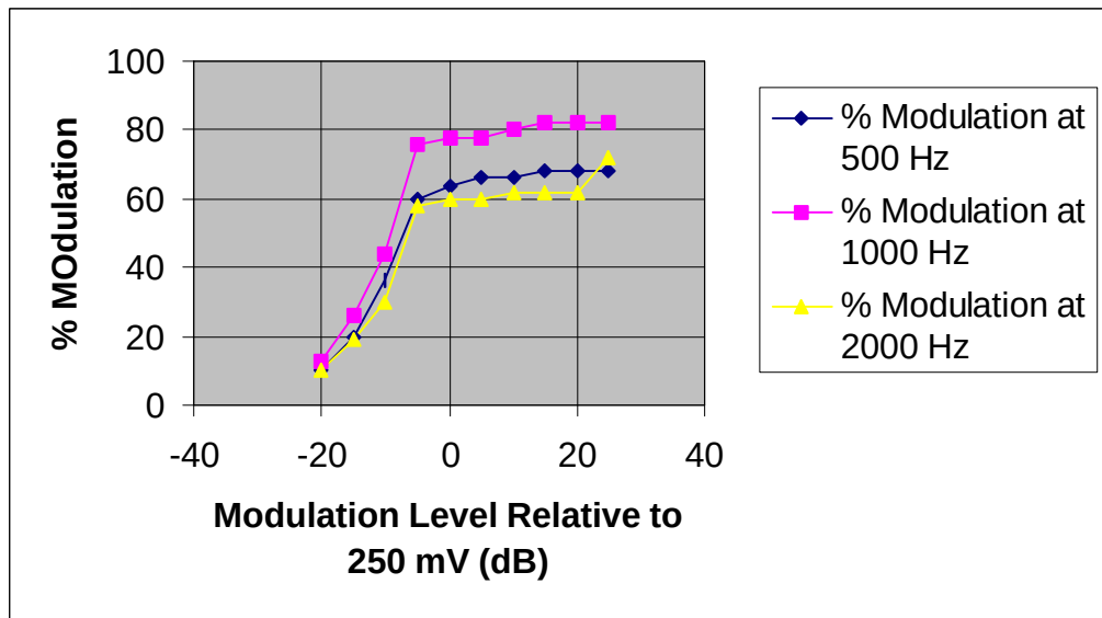
Figure 6: Modulation Characteristics.
