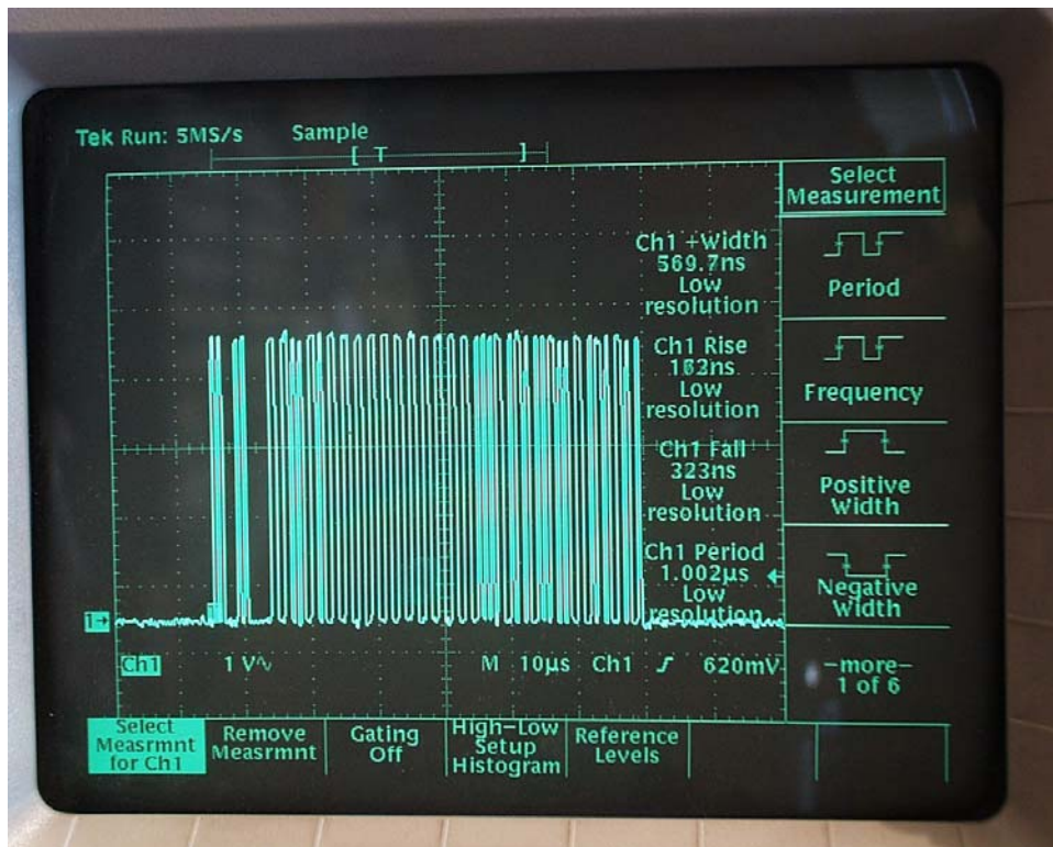
Figure 3 Modulation characteristics
