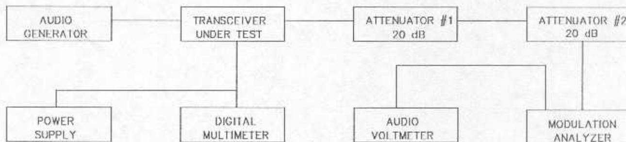
TEST SET-UP
