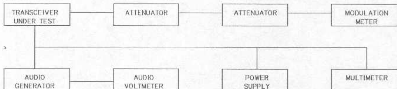
TEST SET-UP
