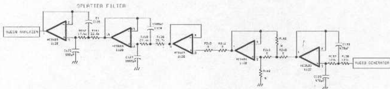
TRANSMIT AUDIO SPLATTER FILTER
