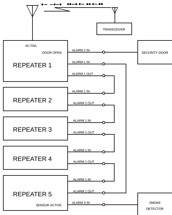
Figure 6-16 ALARM EXAMPLE
