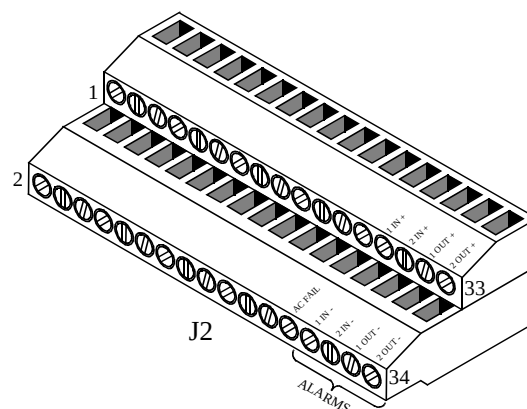
Figure 6-14 4 I/O J2 ALARM OUTPUTS
