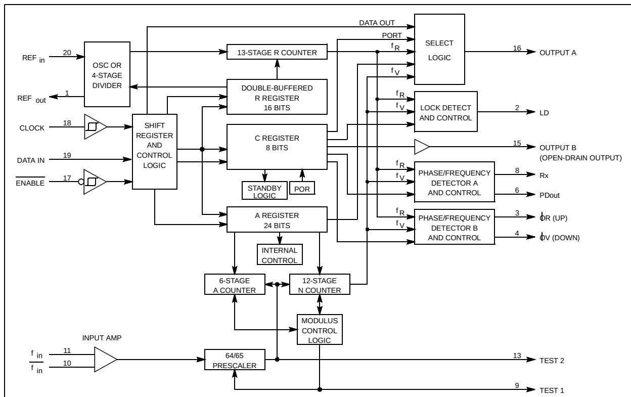
Figure 6-3 SYNTHESIZER BLOCK DIAGRAM
