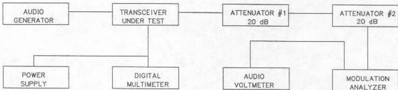
TEST SET-UP
