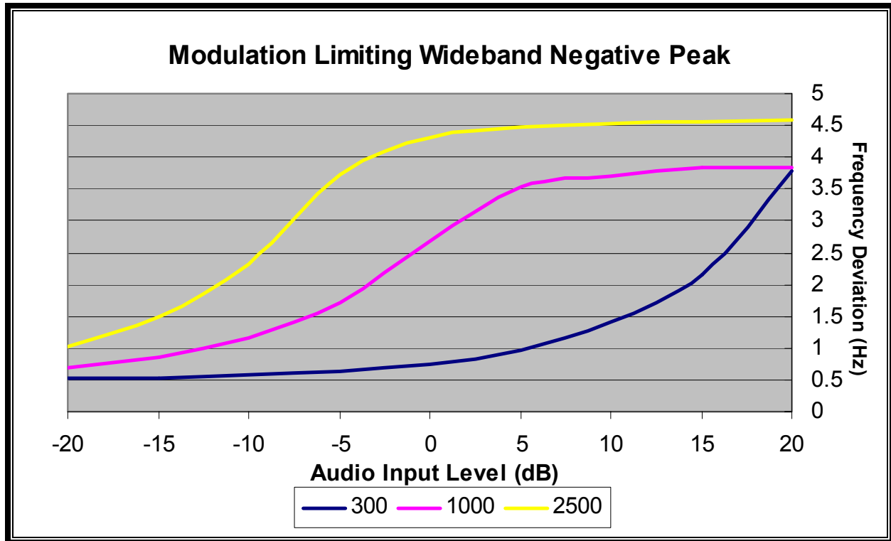
PLOT 8-2: MODULATION LIMITING RESPONSE (WIDEBAND; NEGATIVE PEAK), CH 2, 480 MHZ
