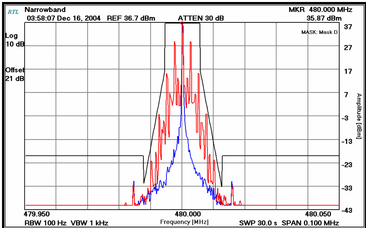
PLOT 9-1: MASK D (480 MHz; CH 5; NARROWBAND)
