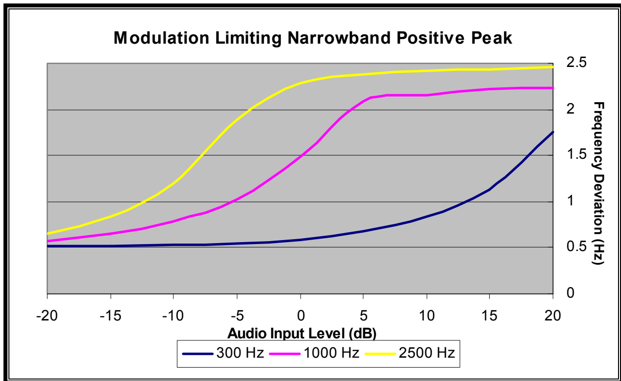
PLOT 8-3: MODULATION LIMITING RESPONSE (NARROWBAND; POSITIVE PEAK), CH 5, 480 MHZ
