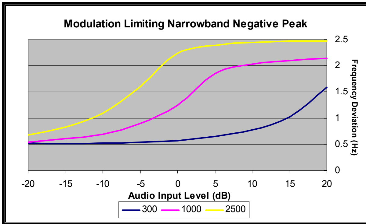
PLOT 8-4: MODULATION LIMITING RESPONSE (NARROWBAND; NEGATIVE PEAK), CH 5, 480 MHZ
