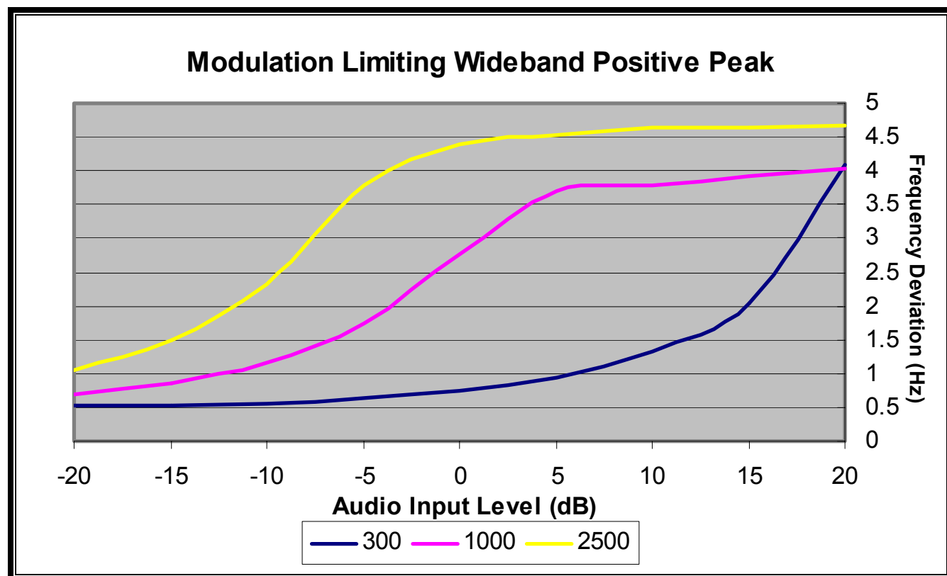
PLOT 8-1: MODULATION LIMITING RESPONSE (WIDEBAND POSITIVE PEAK), CHANNEL 2, 480 MHZ
