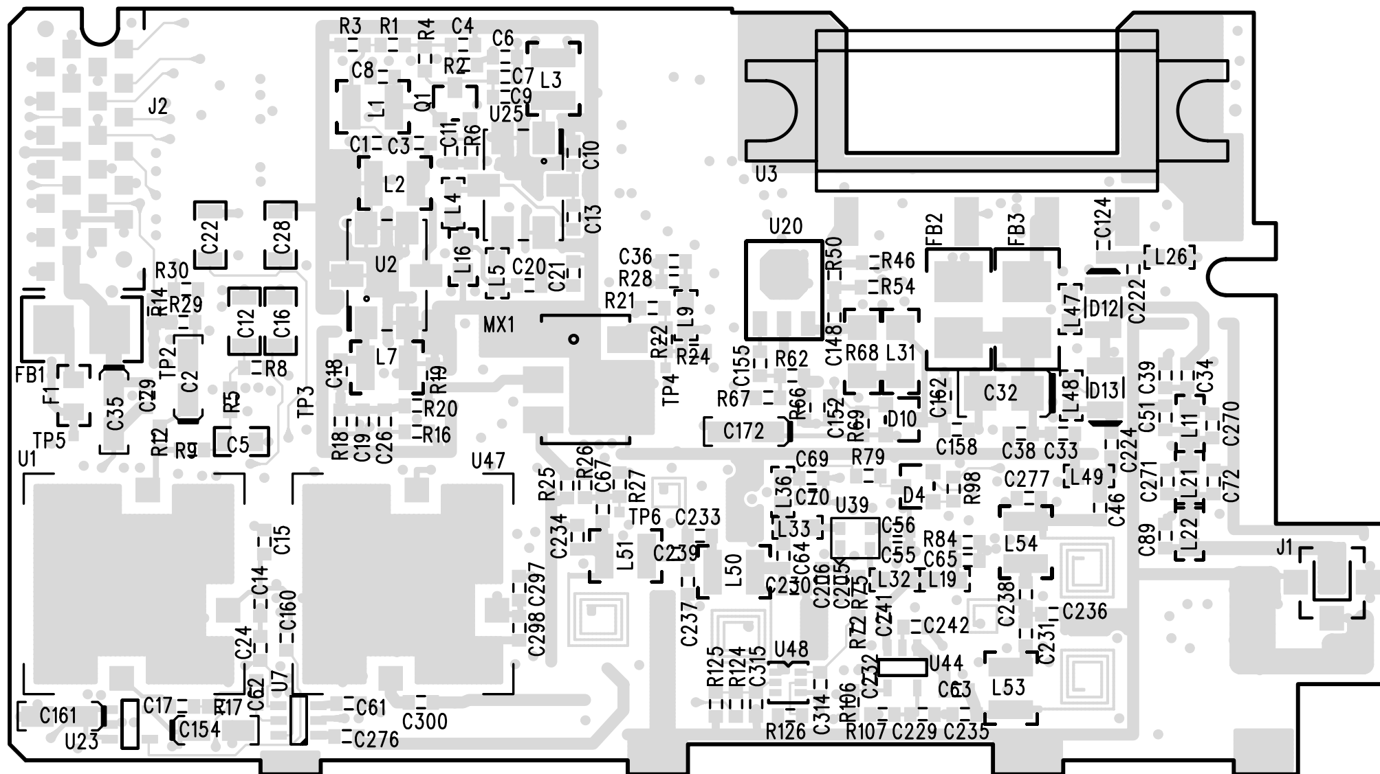
VHF RF BOARD TOP VIEW
