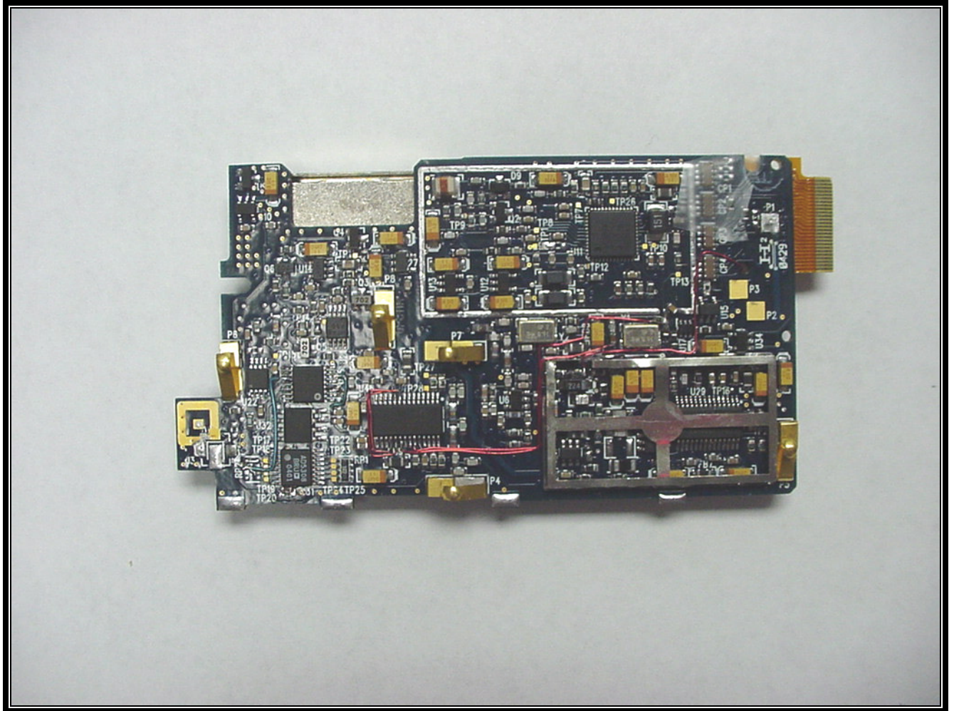
PHOTOGRAPH 18: RF BOARD BOTTOM
