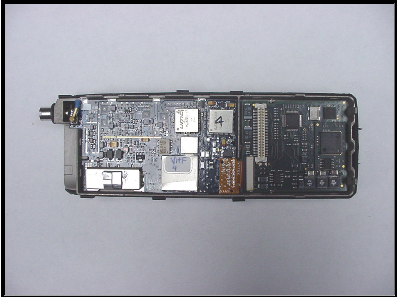
PHOTOGRAPH 14: CHASSIS WITH SHIELDS REMOVED
