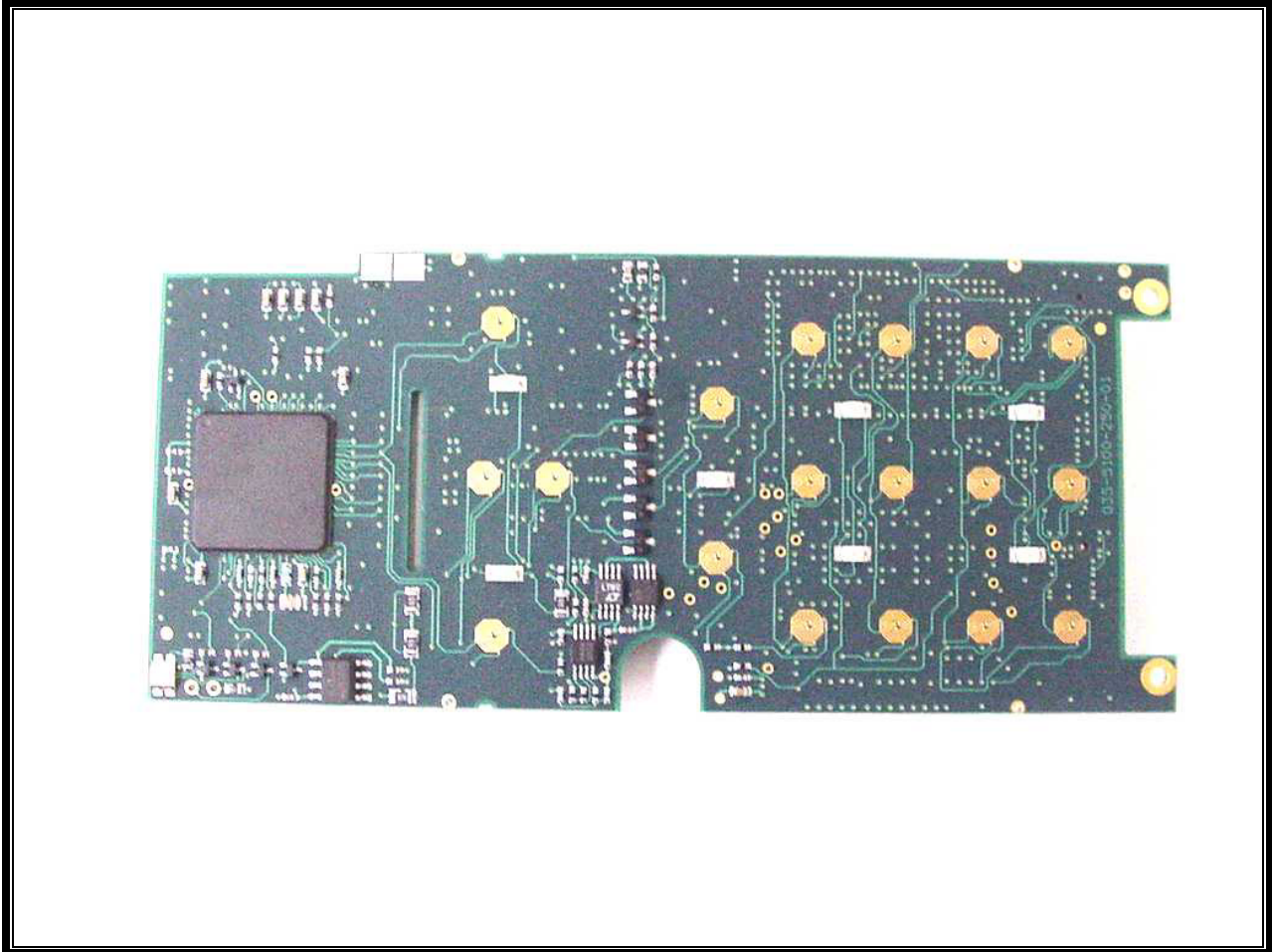
PHOTOGRAPH 22: USER INTERFACE BOARD FRONT
