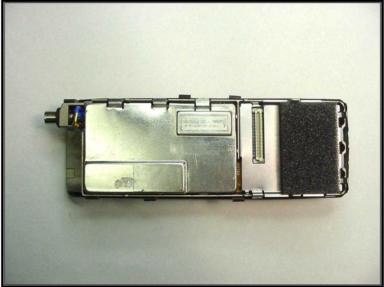
PHOTOGRAPH 13: CHASSIS WITH SHIELDS
