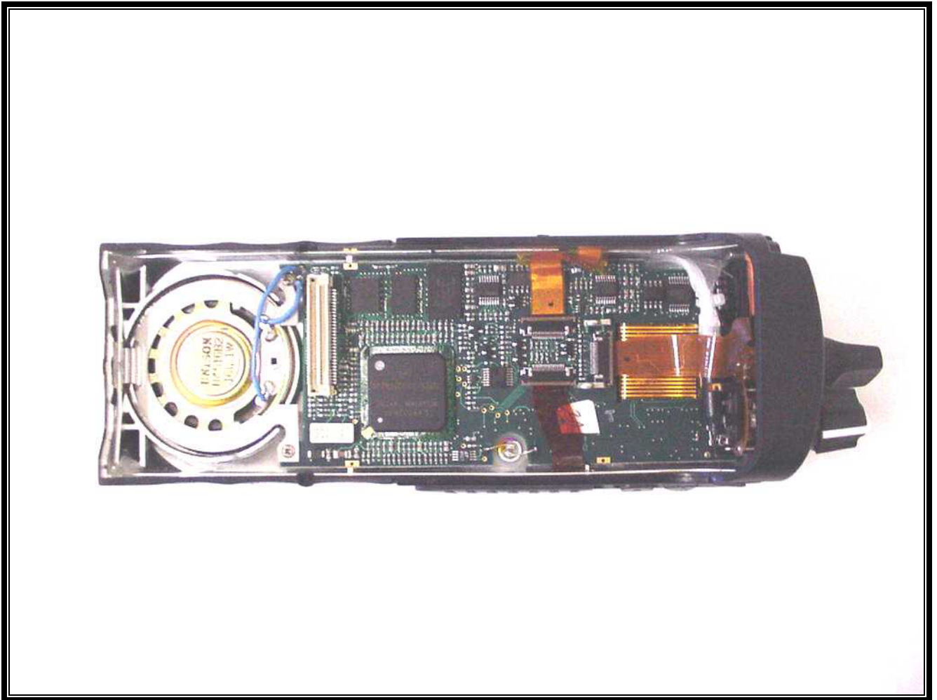
PHOTOGRAPH 20: USER INTERFACE BOARD IN FRONT COVER
