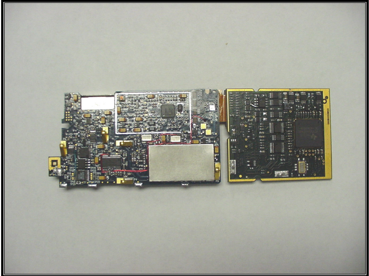
PHOTOGRAPH 15: RF AND LOGIC BOARD BACK OUT OF CHASSIS
