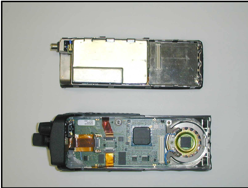
PHOTOGRAPH 12: OPEN SHIELDS VIEW
