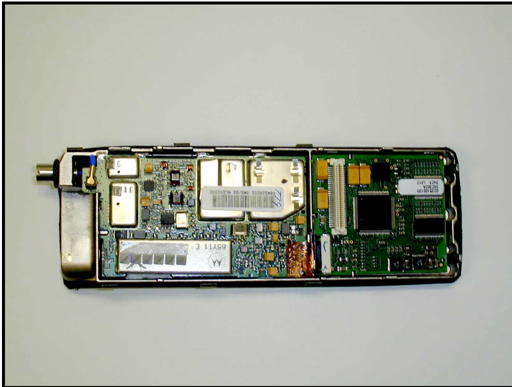
PHOTOGRAPH 10: BOARDS TOP VIEW
